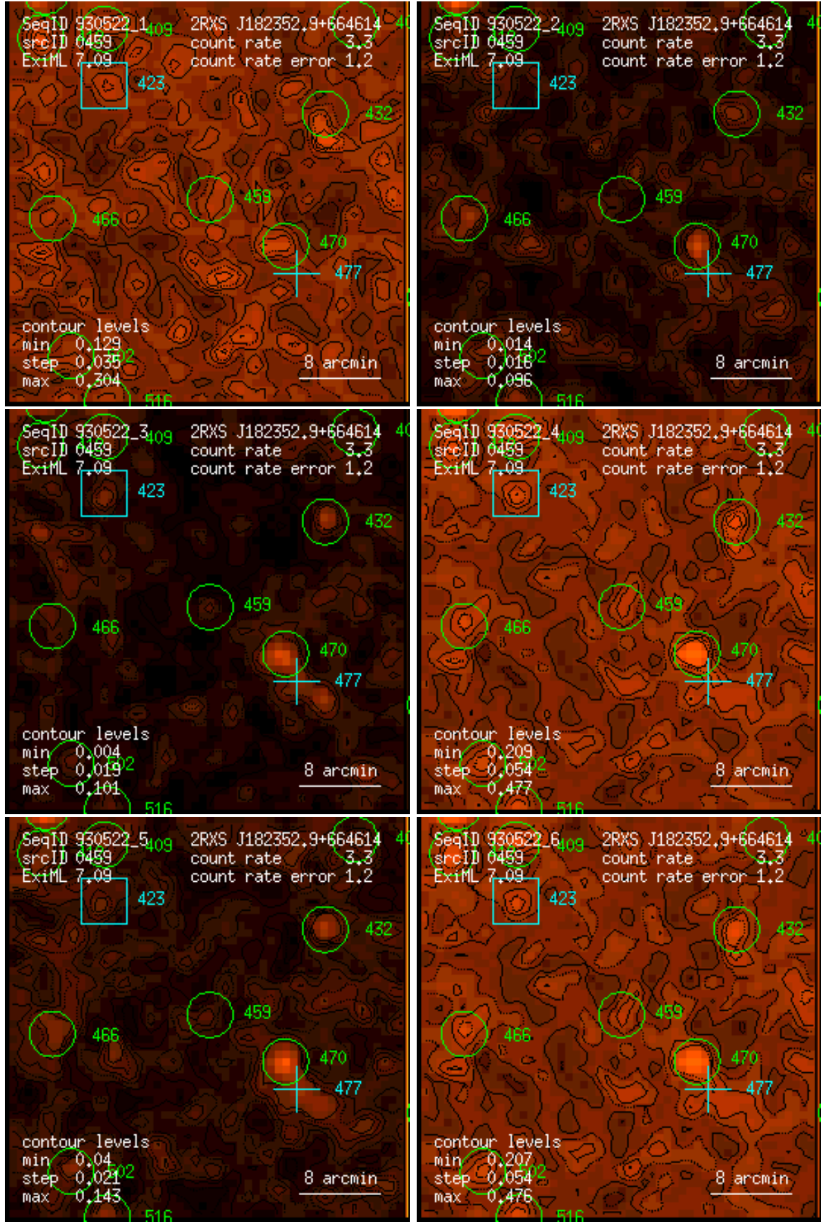
Figure 459: RASS 930522: detection 0459: band rate images, Gaussian filter: (1) PSPC channels 11 – 41, (2) 52 – 90, (3) 91 – 201, (4) 11 – 235, (5) 52 – 201, (6) 11 – 201. Broad band rates in counts/ks. Band rate contour levels in counts/ks/arcmin 2 .
