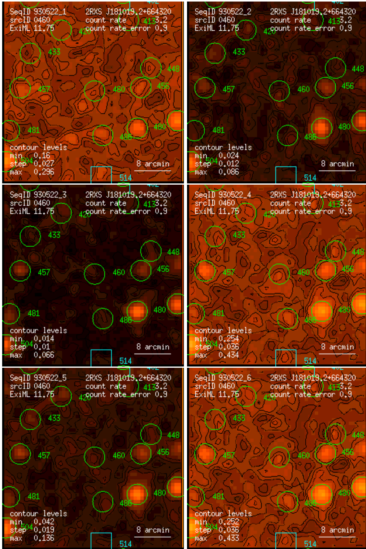
Figure 460: RASS 930522: detection 0460: band rate images, Gaussian filter: (1) PSPC channels 11 – 41, (2) 52 – 90, (3) 91 – 201, (4) 11 – 235, (5) 52 – 201, (6) 11 – 201. Broad band rates in counts/ks. Band rate contour levels in counts/ks/arcmin 2 .
