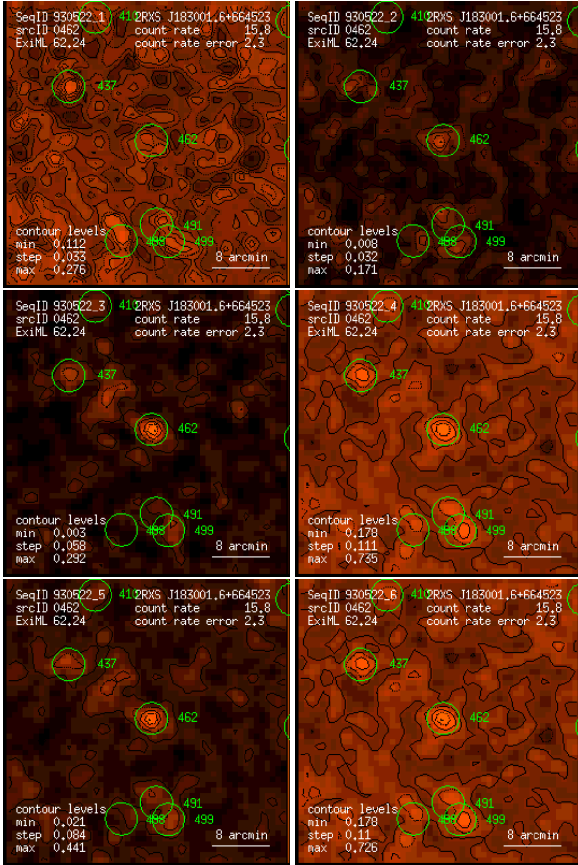
Figure 462: RASS 930522: detection 0462: band rate images, Gaussian filter: (1) PSPC channels 11 – 41, (2) 52 – 90, (3) 91 – 201, (4) 11 – 235, (5) 52 – 201, (6) 11 – 201. Broad band rates in counts/ks. Band rate contour levels in counts/ks/arcmin 2 .
