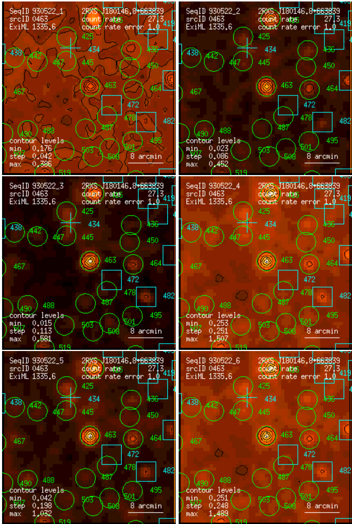
Figure 463: RASS 930522: detection 0463: band rate images, Gaussian filter: (1) PSPC channels 11 – 41, (2) 52 – 90, (3) 91 – 201, (4) 11 – 235, (5) 52 – 201, (6) 11 – 201. Broad band rates in counts/ks. Band rate contour levels in counts/ks/arcmin 2 .
