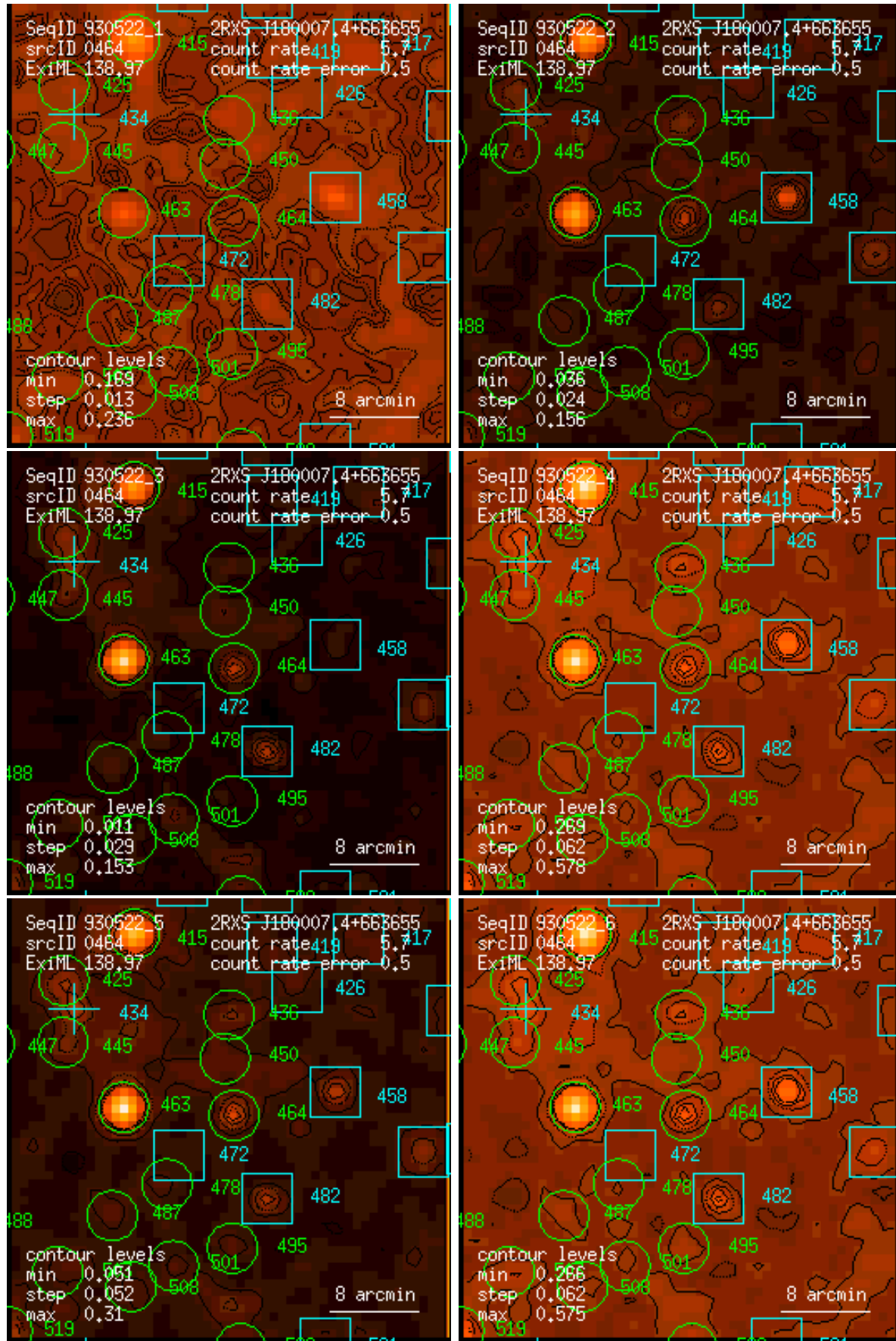
Figure 464: RASS 930522: detection 0464: band rate images, Gaussian filter: (1) PSPC channels 11 – 41, (2) 52 – 90, (3) 91 – 201, (4) 11 – 235, (5) 52 – 201, (6) 11 – 201. Broad band rates in counts/ks. Band rate contour levels in counts/ks/arcmin 2 .
