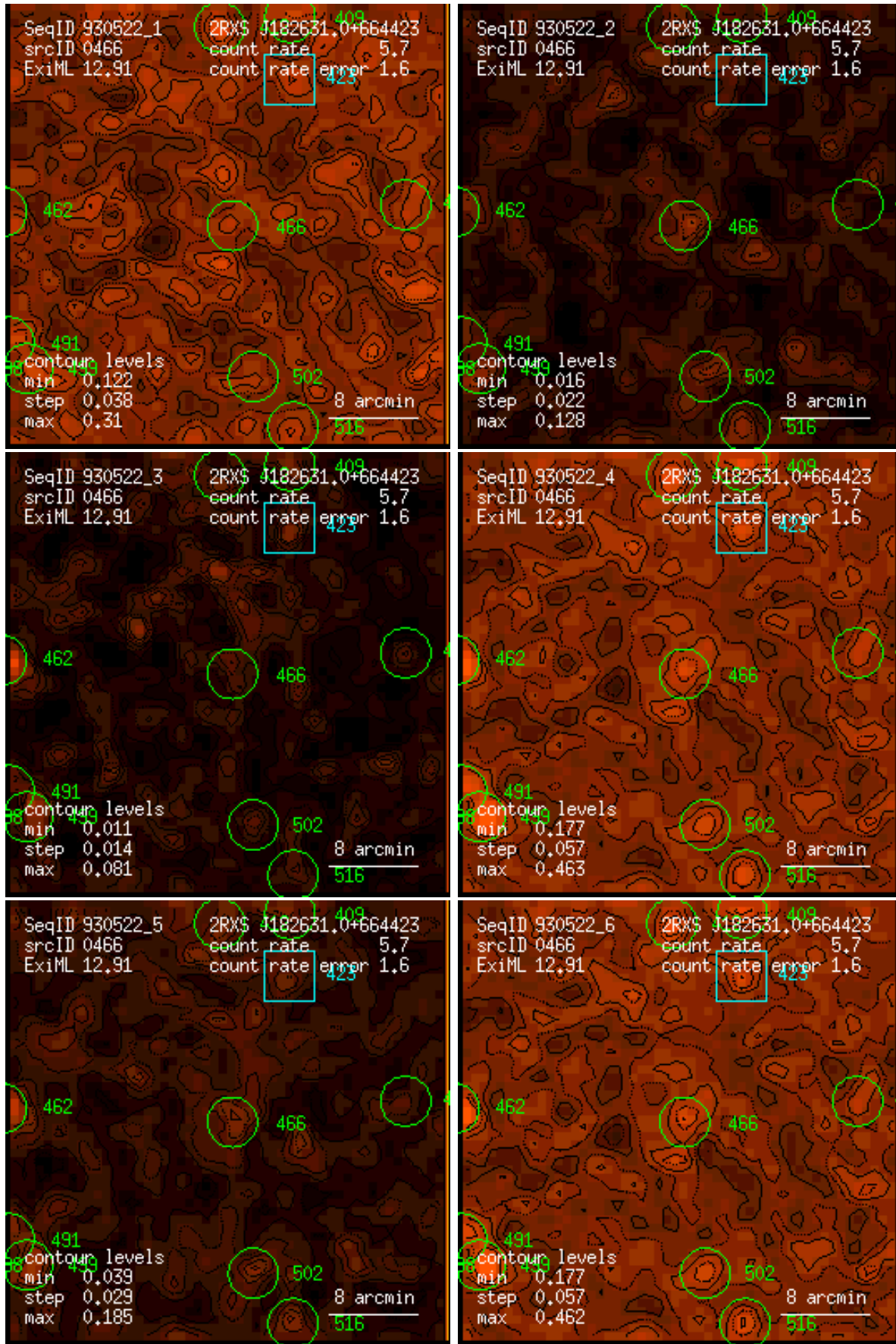
Figure 466: RASS 930522: detection 0466: band rate images, Gaussian filter: (1) PSPC channels 11 – 41, (2) 52 – 90, (3) 91 – 201, (4) 11 – 235, (5) 52 – 201, (6) 11 – 201. Broad band rates in counts/ks. Band rate contour levels in counts/ks/arcmin 2 .
