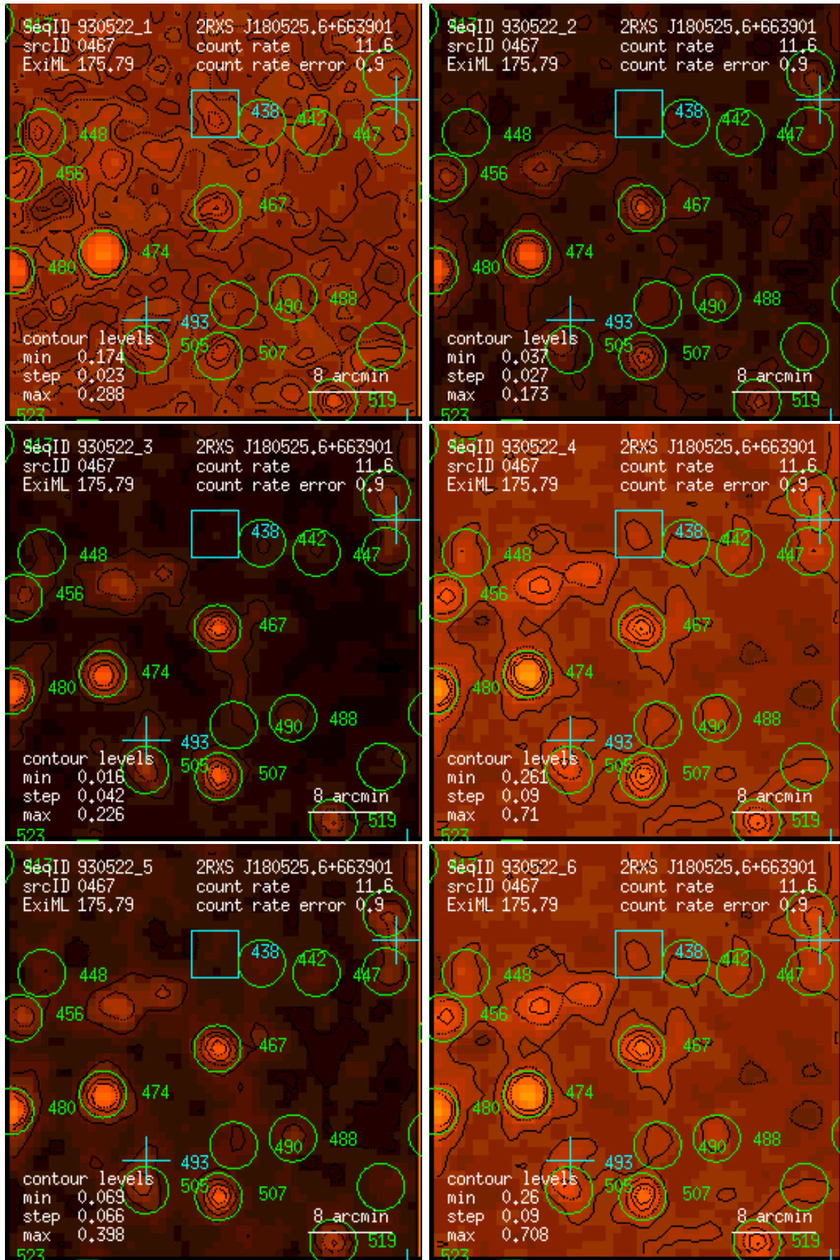
Figure 467: RASS 930522: detection 0467: band rate images, Gaussian filter: (1) PSPC channels 11 – 41, (2) 52 – 90, (3) 91 – 201, (4) 11 – 235, (5) 52 – 201, (6) 11 – 201. Broad band rates in counts/ks. Band rate contour levels in counts/ks/arcmin 2 .
