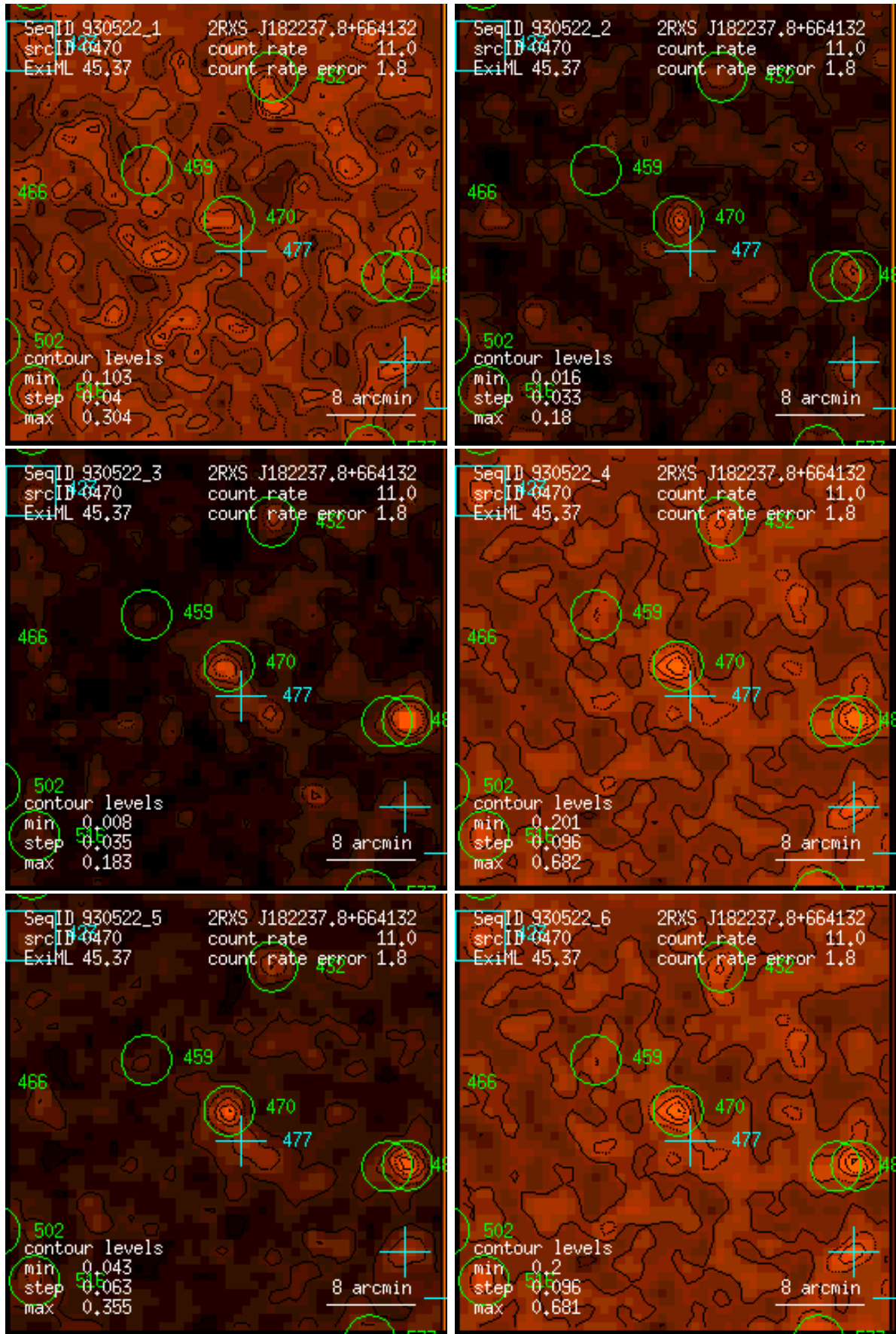
Figure 470: RASS 930522: detection 0470: band rate images, Gaussian filter: (1) PSPC channels 11 – 41, (2) 52 – 90, (3) 91 – 201, (4) 11 – 235, (5) 52 – 201, (6) 11 – 201. Broad band rates in counts/ks. Band rate contour levels in counts/ks/arcmin 2 .
