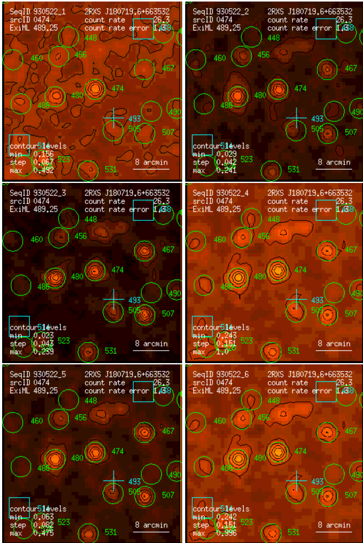
Figure 474: RASS 930522: detection 0474: band rate images, Gaussian filter: (1) PSPC channels 11 – 41, (2) 52 – 90, (3) 91 – 201, (4) 11 – 235, (5) 52 – 201, (6) 11 – 201. Broad band rates in counts/ks. Band rate contour levels in counts/ks/arcmin 2 .
