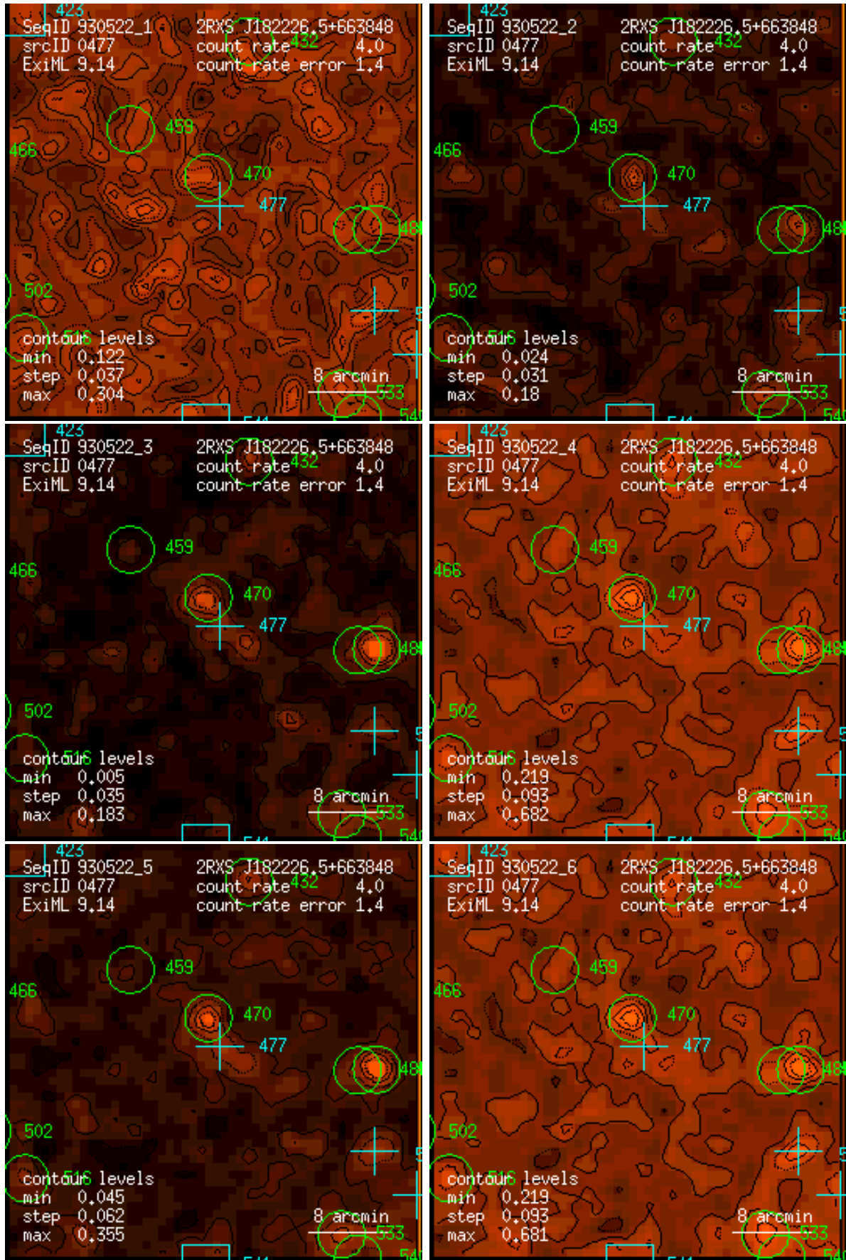
Figure 477: RASS 930522: detection 0477: band rate images, Gaussian filter: (1) PSPC channels 11 – 41, (2) 52 – 90, (3) 91 – 201, (4) 11 – 235, (5) 52 – 201, (6) 11 – 201. Broad band rates in counts/ks. Band rate contour levels in counts/ks/arcmin 2 .
