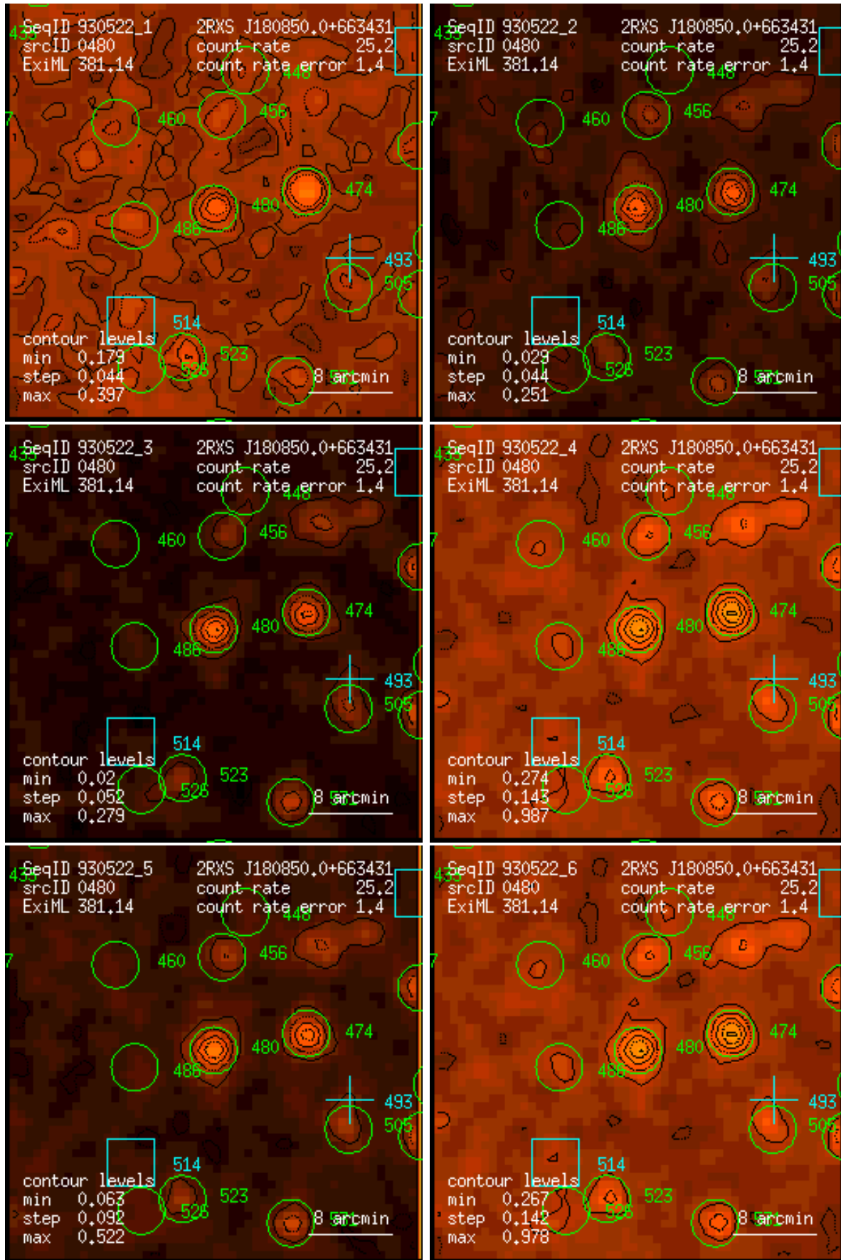
Figure 480: RASS 930522: detection 0480: band rate images, Gaussian filter: (1) PSPC channels 11 – 41, (2) 52 – 90, (3) 91 – 201, (4) 11 – 235, (5) 52 – 201, (6) 11 – 201. Broad band rates in counts/ks. Band rate contour levels in counts/ks/arcmin 2 .
