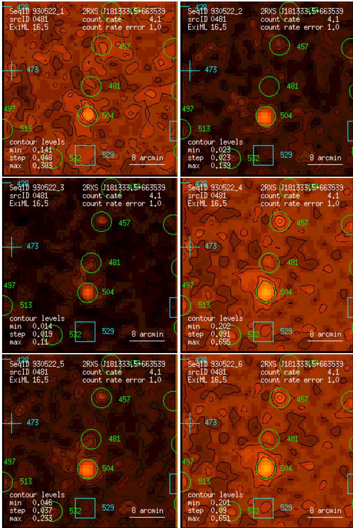
Figure 481: RASS 930522: detection 0481: band rate images, Gaussian filter: (1) PSPC channels 11 – 41, (2) 52 – 90, (3) 91 – 201, (4) 11 – 235, (5) 52 – 201, (6) 11 – 201. Broad band rates in counts/ks. Band rate contour levels in counts/ks/arcmin 2 .
