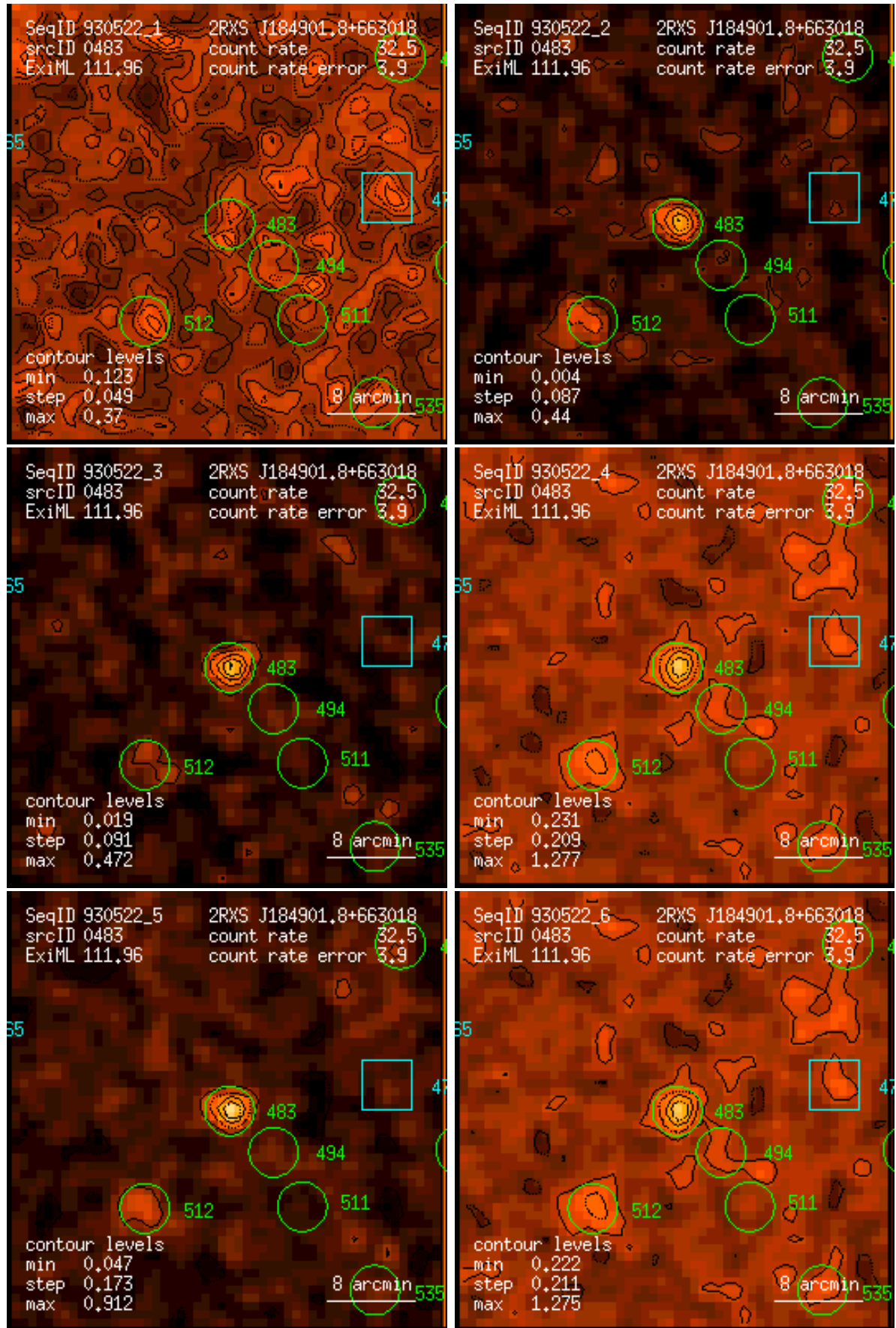
Figure 483: RASS 930522: detection 0483: band rate images, Gaussian filter: (1) PSPC channels 11 – 41, (2) 52 – 90, (3) 91 – 201, (4) 11 – 235, (5) 52 – 201, (6) 11 – 201. Broad band rates in counts/ks. Band rate contour levels in counts/ks/arcmin 2 .
