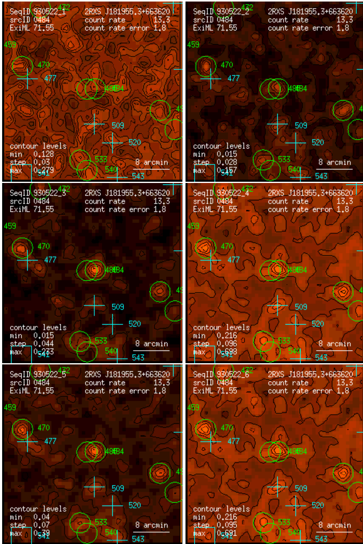
Figure 484: RASS 930522: detection 0484: band rate images, Gaussian filter: (1) PSPC channels 11 – 41, (2) 52 – 90, (3) 91 – 201, (4) 11 – 235, (5) 52 – 201, (6) 11 – 201. Broad band rates in counts/ks. Band rate contour levels in counts/ks/arcmin 2 .
