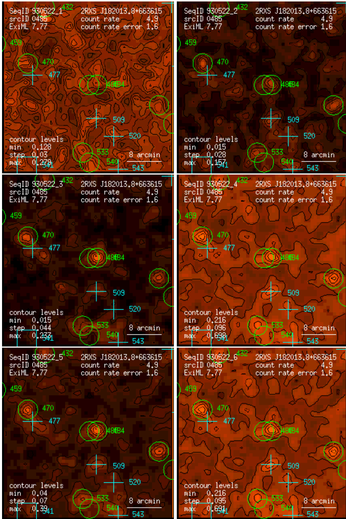
Figure 485: RASS 930522: detection 0485: band rate images, Gaussian filter: (1) PSPC channels 11 – 41, (2) 52 – 90, (3) 91 – 201, (4) 11 – 235, (5) 52 – 201, (6) 11 – 201. Broad band rates in counts/ks. Band rate contour levels in counts/ks/arcmin 2 .
