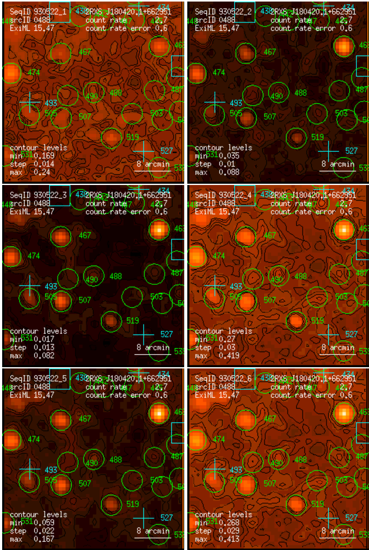
Figure 488: RASS 930522: detection 0488: band rate images, Gaussian filter: (1) PSPC channels 11 – 41, (2) 52 – 90, (3) 91 – 201, (4) 11 – 235, (5) 52 – 201, (6) 11 – 201. Broad band rates in counts/ks. Band rate contour levels in counts/ks/arcmin 2 .
