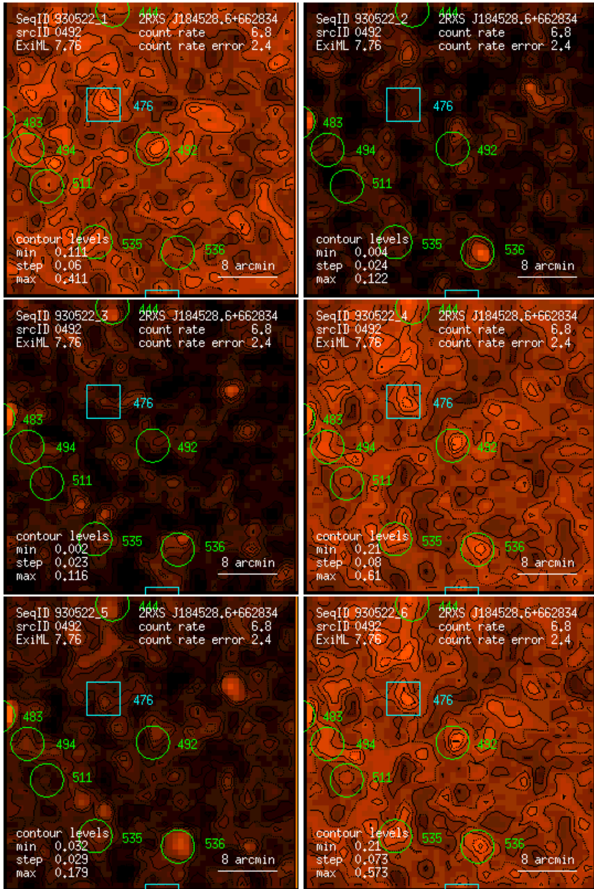
Figure 492: RASS 930522: detection 0492: band rate images, Gaussian filter: (1) PSPC channels 11 – 41, (2) 52 – 90, (3) 91 – 201, (4) 11 – 235, (5) 52 – 201, (6) 11 – 201. Broad band rates in counts/ks. Band rate contour levels in counts/ks/arcmin 2 .
