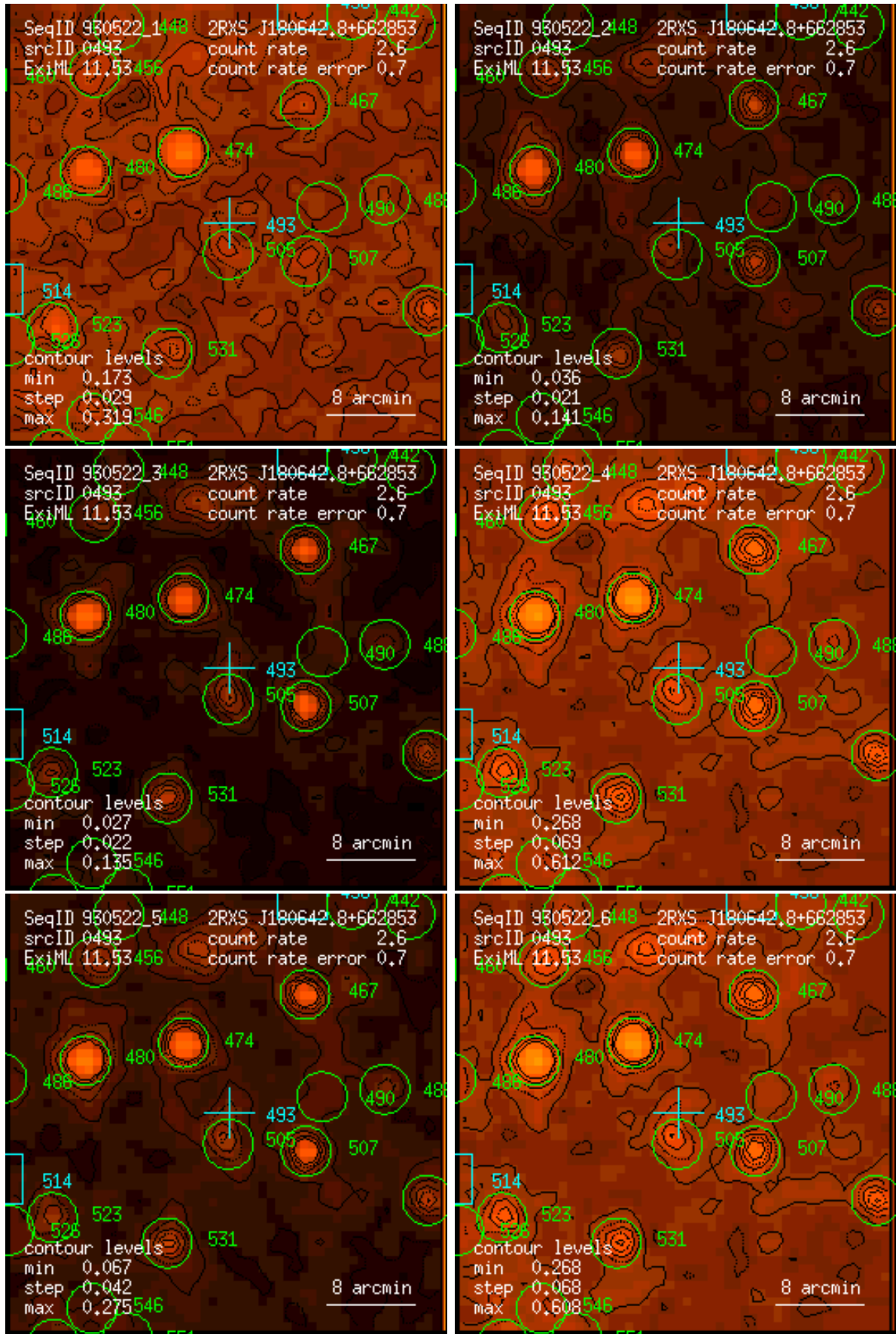
Figure 493: RASS 930522: detection 0493: band rate images, Gaussian filter: (1) PSPC channels 11 – 41, (2) 52 – 90, (3) 91 – 201, (4) 11 – 235, (5) 52 – 201, (6) 11 – 201. Broad band rates in counts/ks. Band rate contour levels in counts/ks/arcmin 2 .
