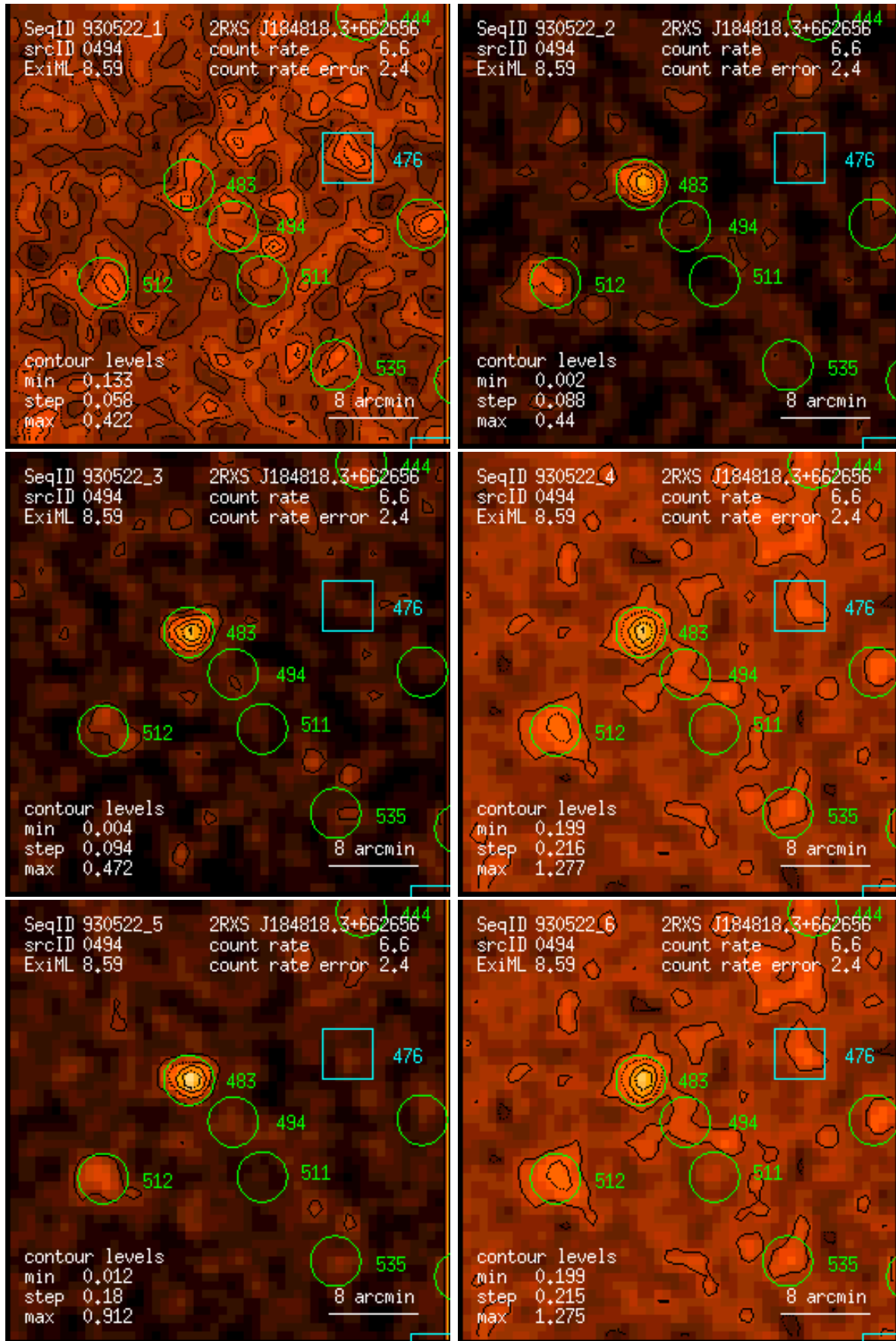
Figure 494: RASS 930522: detection 0494: band rate images, Gaussian filter: (1) PSPC channels 11 – 41, (2) 52 – 90, (3) 91 – 201, (4) 11 – 235, (5) 52 – 201, (6) 11 – 201. Broad band rates in counts/ks. Band rate contour levels in counts/ks/arcmin 2 .
