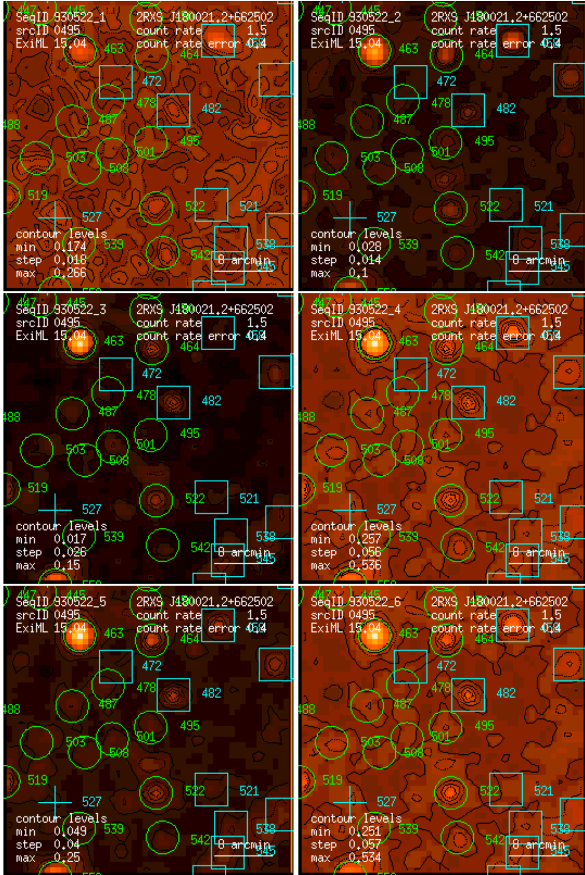
Figure 495: RASS 930522: detection 0495: band rate images, Gaussian filter: (1) PSPC channels 11 – 41, (2) 52 – 90, (3) 91 – 201, (4) 11 – 235, (5) 52 – 201, (6) 11 – 201. Broad band rates in counts/ks. Band rate contour levels in counts/ks/arcmin 2 .
