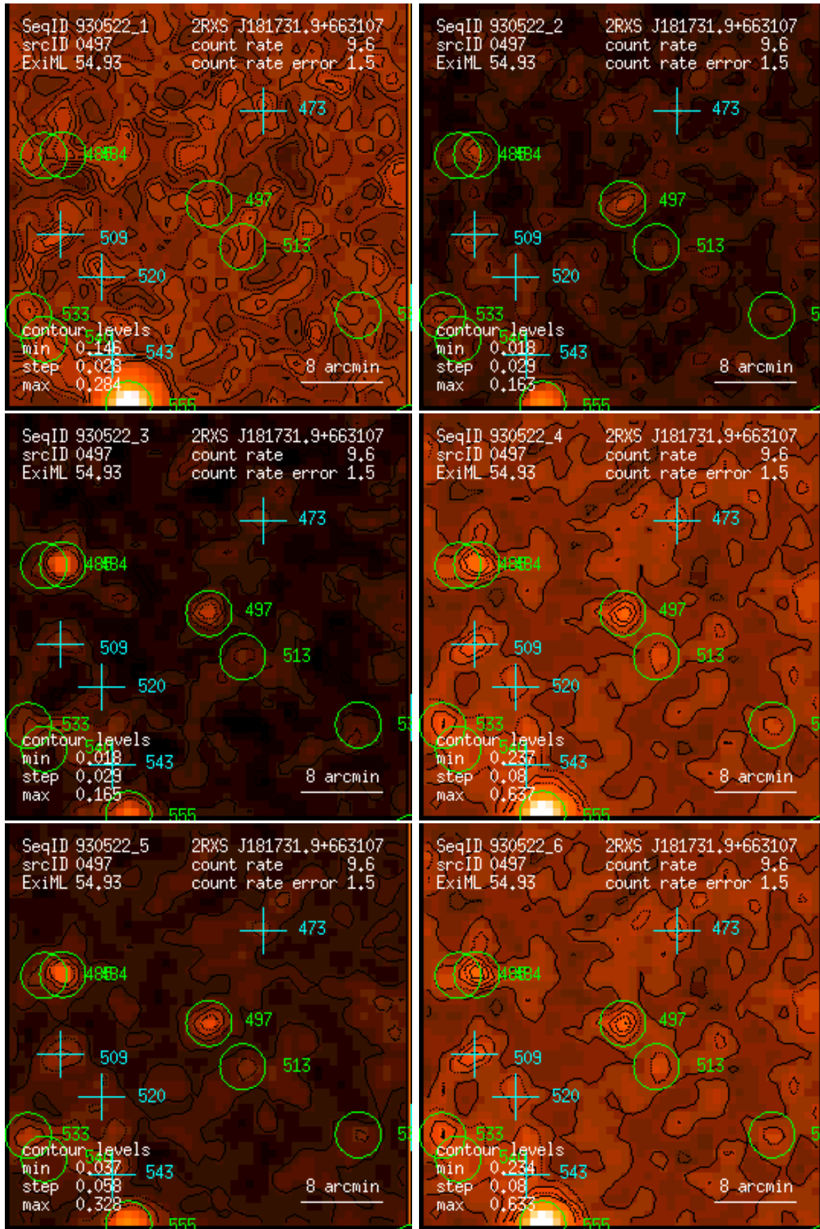
Figure 497: RASS 930522: detection 0497: band rate images, Gaussian filter: (1) PSPC channels 11 – 41, (2) 52 – 90, (3) 91 – 201, (4) 11 – 235, (5) 52 – 201, (6) 11 – 201. Broad band rates in counts/ks. Band rate contour levels in counts/ks/arcmin 2 .
