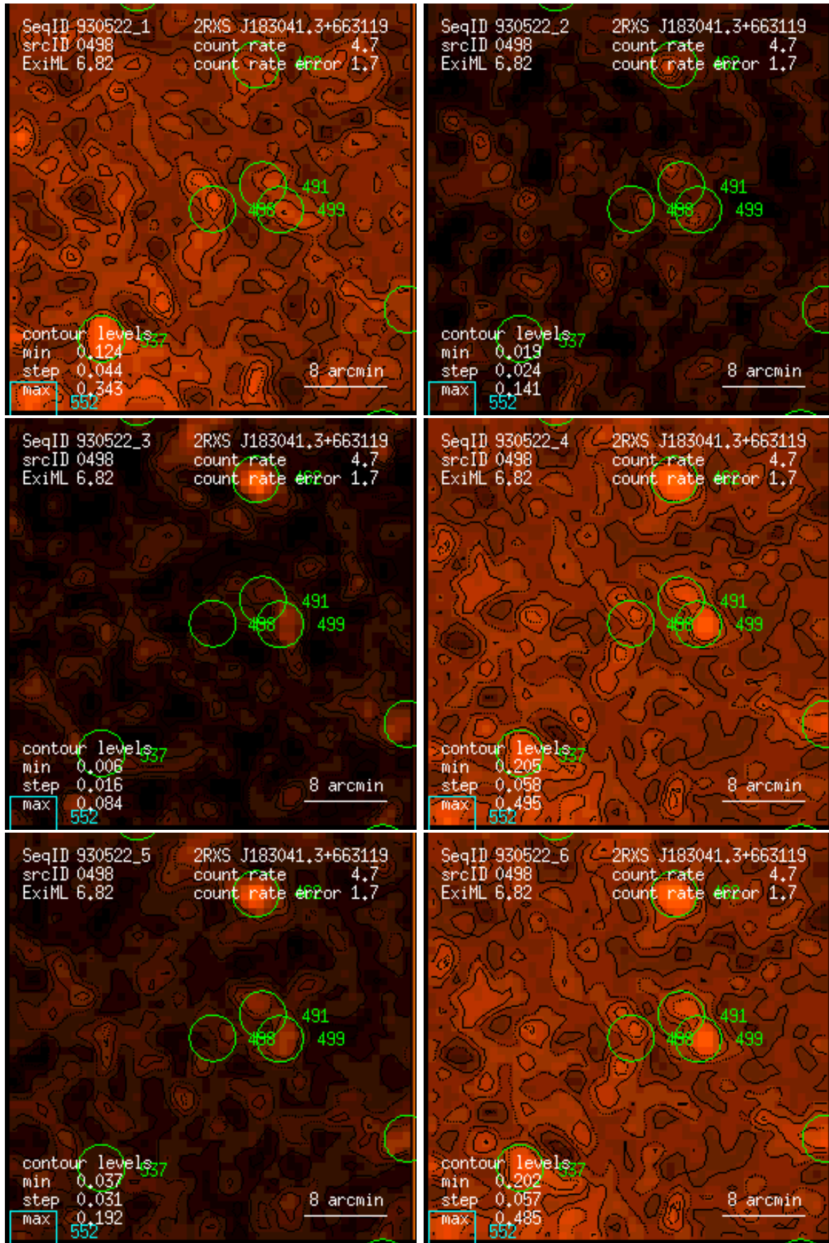
Figure 498: RASS 930522: detection 0498: band rate images, Gaussian filter: (1) PSPC channels 11 – 41, (2) 52 – 90, (3) 91 – 201, (4) 11 – 235, (5) 52 – 201, (6) 11 – 201. Broad band rates in counts/ks. Band rate contour levels in counts/ks/arcmin 2 .
