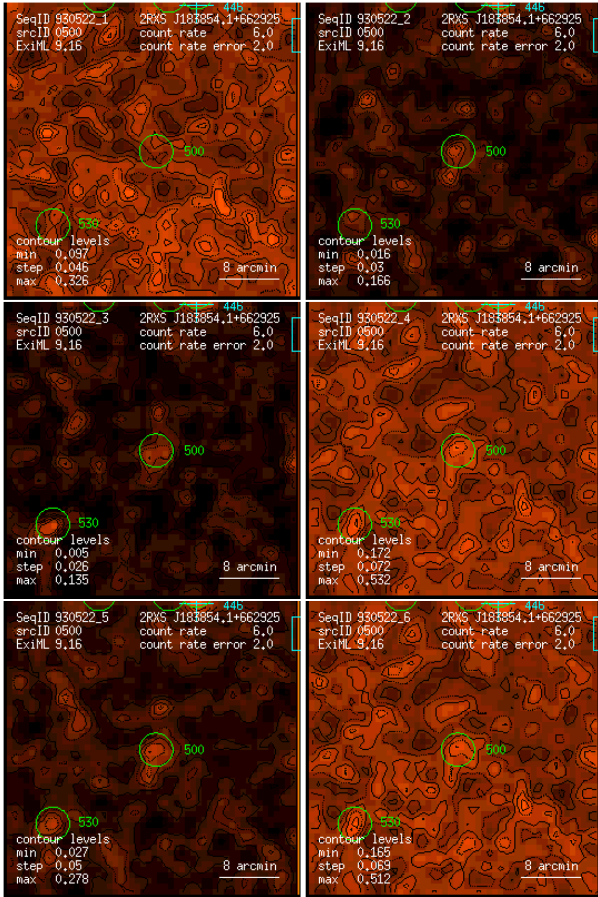
Figure 500: RASS 930522: detection 0500: band rate images, Gaussian filter: (1) PSPC channels 11 – 41, (2) 52 – 90, (3) 91 – 201, (4) 11 – 235, (5) 52 – 201, (6) 11 – 201. Broad band rates in counts/ks. Band rate contour levels in counts/ks/arcmin 2 .
