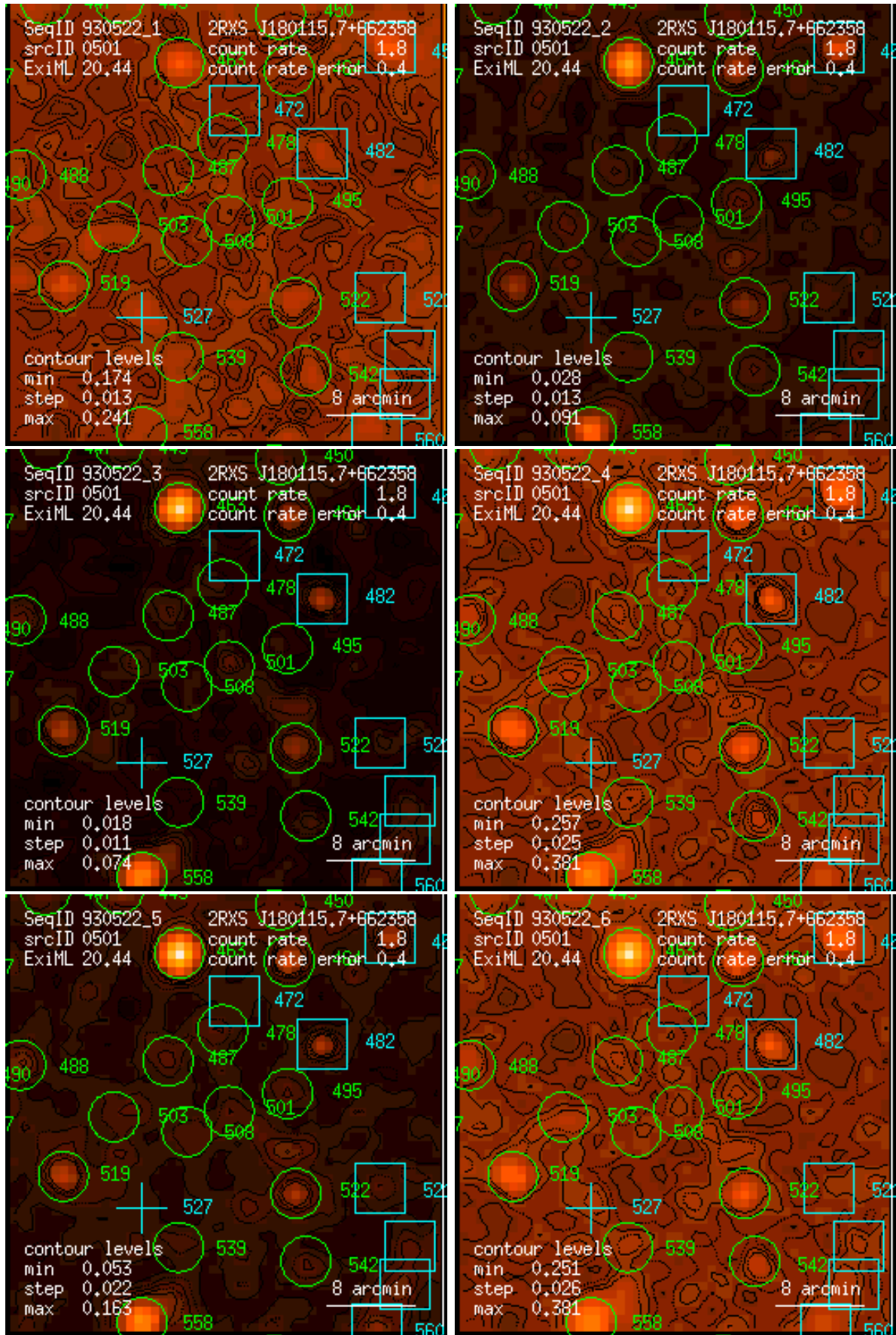
Figure 501: RASS 930522: detection 0501: band rate images, Gaussian filter: (1) PSPC channels 11 – 41, (2) 52 – 90, (3) 91 – 201, (4) 11 – 235, (5) 52 – 201, (6) 11 – 201. Broad band rates in counts/ks. Band rate contour levels in counts/ks/arcmin 2 .
