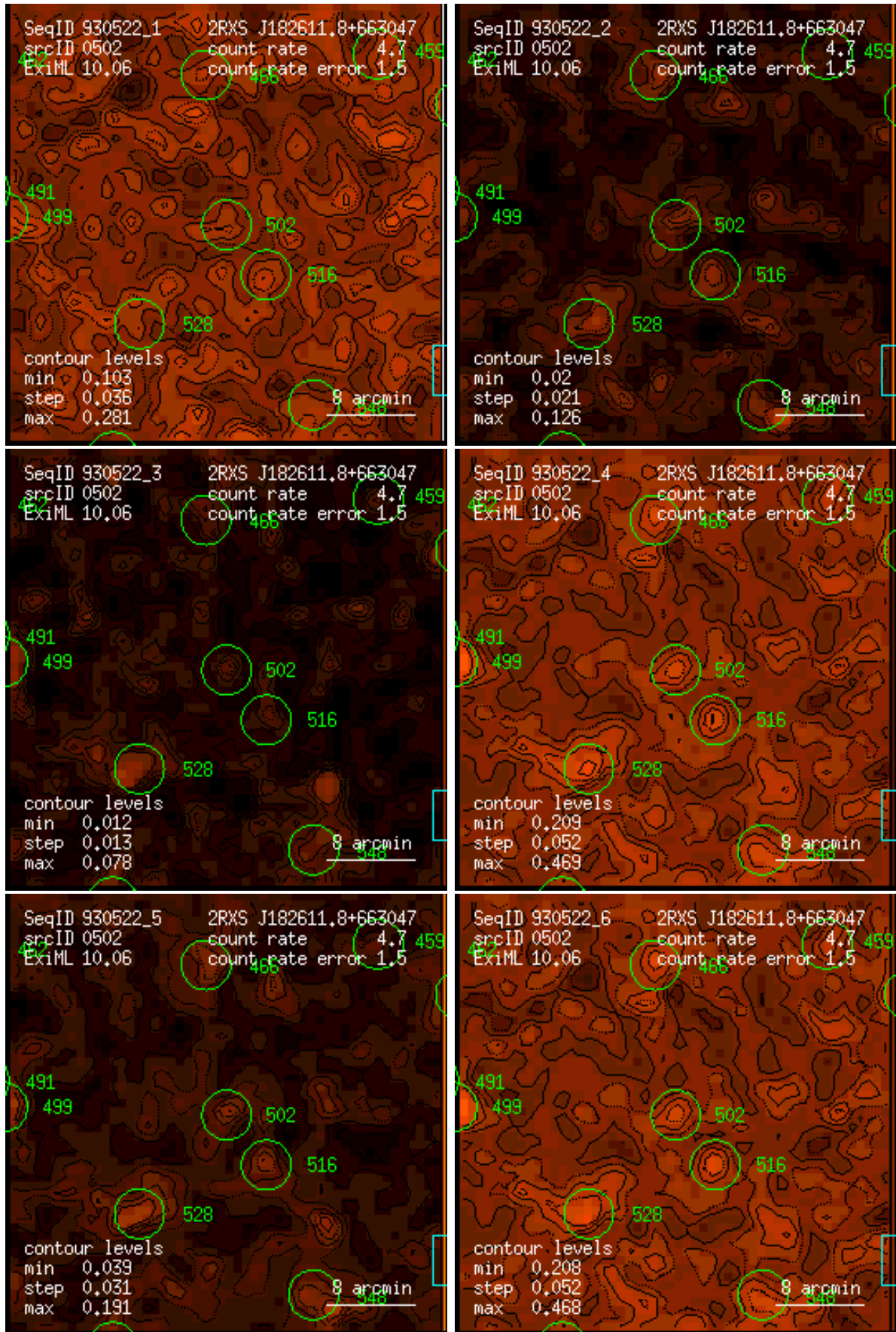
Figure 502: RASS 930522: detection 0502: band rate images, Gaussian filter: (1) PSPC channels 11 – 41, (2) 52 – 90, (3) 91 – 201, (4) 11 – 235, (5) 52 – 201, (6) 11 – 201. Broad band rates in counts/ks. Band rate contour levels in counts/ks/arcmin 2 .
