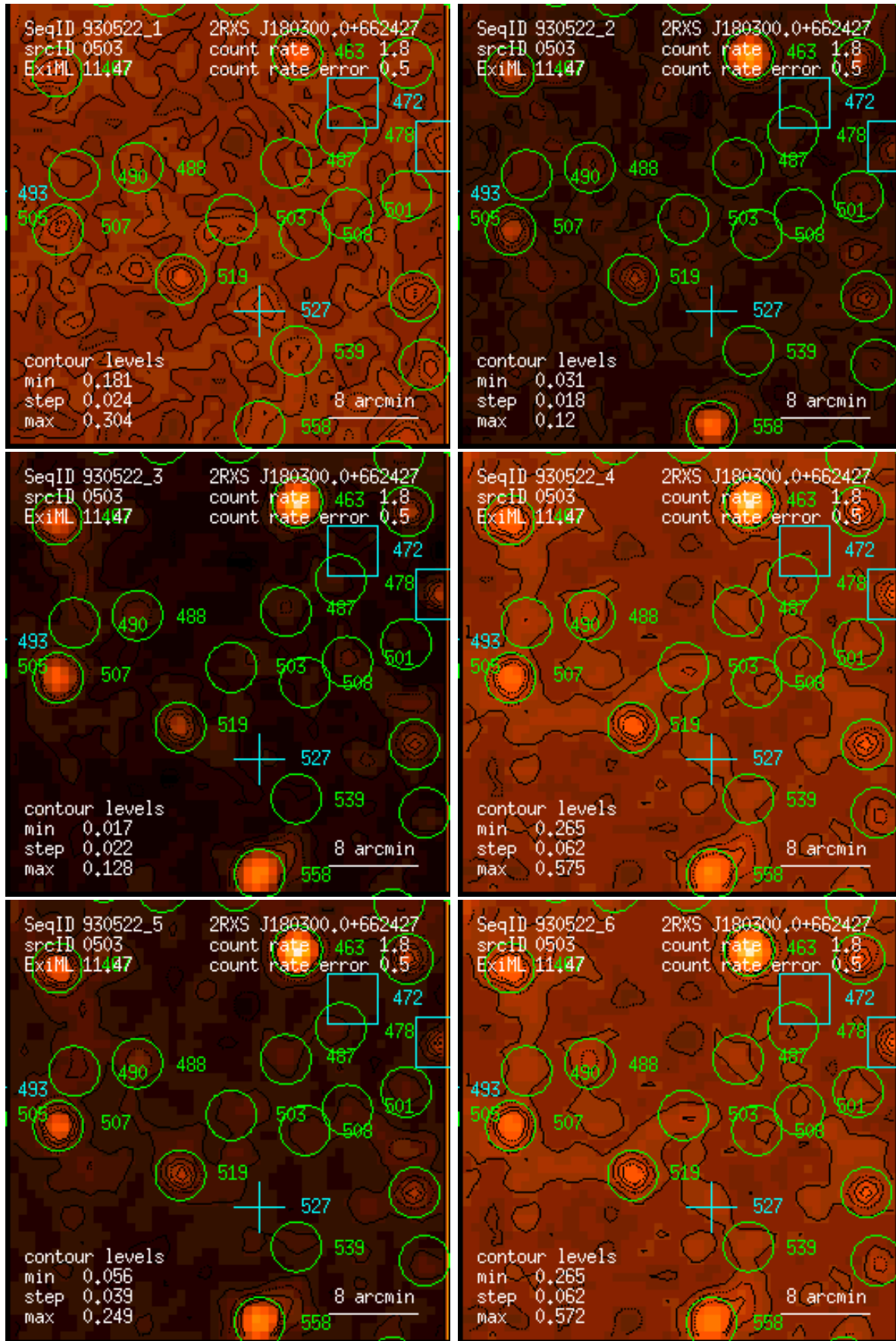
Figure 503: RASS 930522: detection 0503: band rate images, Gaussian filter: (1) PSPC channels 11 – 41, (2) 52 – 90, (3) 91 – 201, (4) 11 – 235, (5) 52 – 201, (6) 11 – 201. Broad band rates in counts/ks. Band rate contour levels in counts/ks/arcmin 2 .
