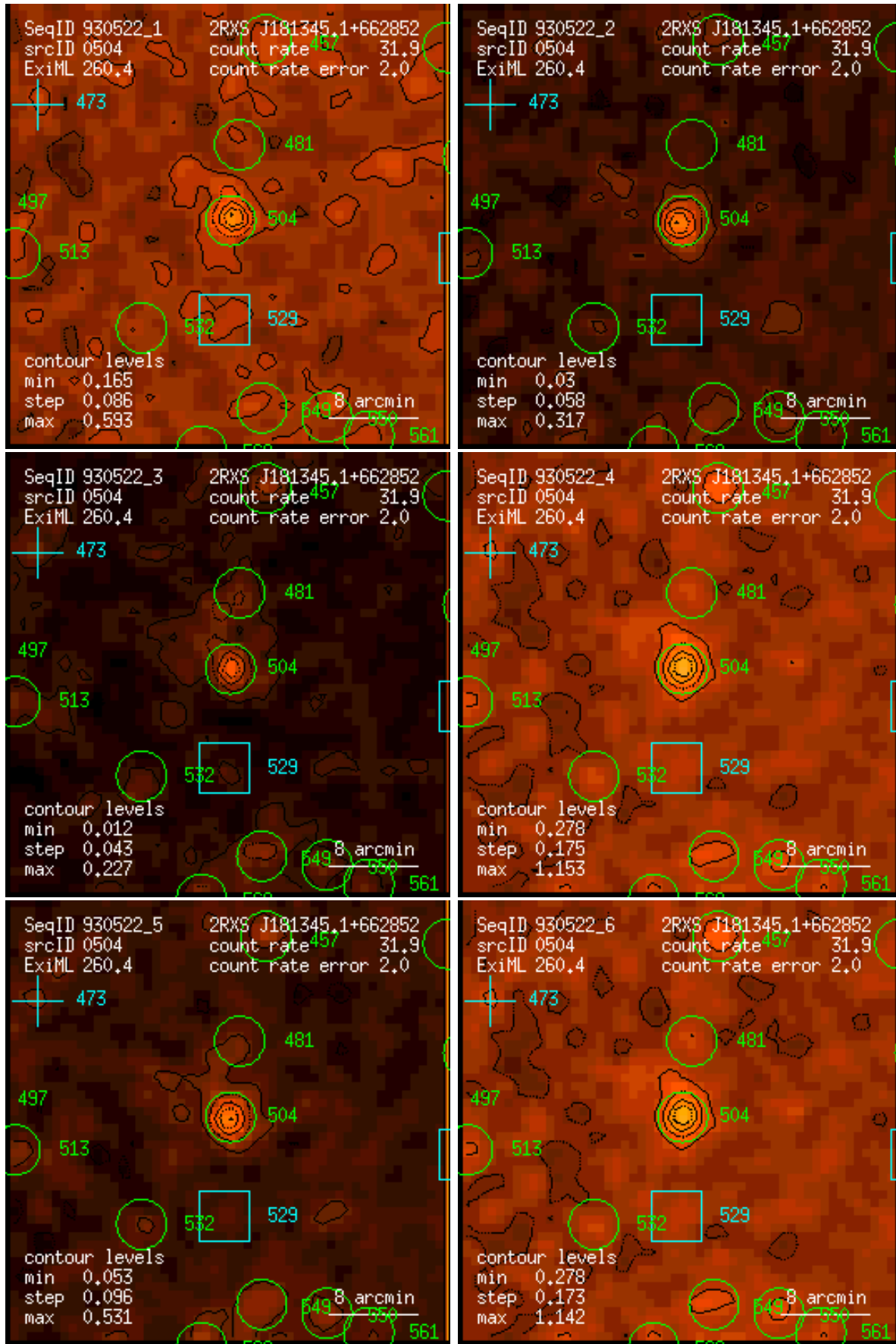
Figure 504: RASS 930522: detection 0504: band rate images, Gaussian filter: (1) PSPC channels 11 – 41, (2) 52 – 90, (3) 91 – 201, (4) 11 – 235, (5) 52 – 201, (6) 11 – 201. Broad band rates in counts/ks. Band rate contour levels in counts/ks/arcmin 2 .
