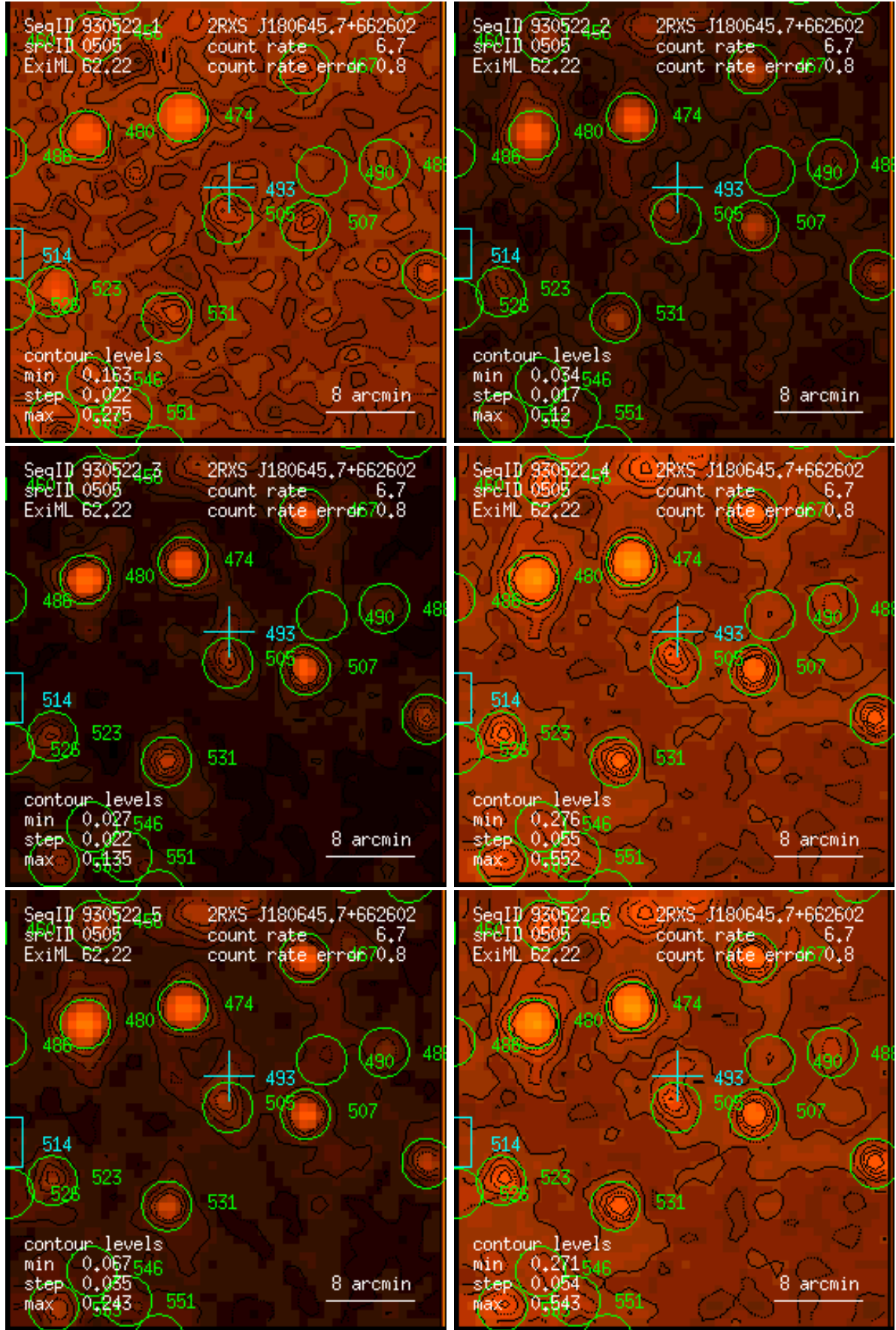
Figure 505: RASS 930522: detection 0505: band rate images, Gaussian filter: (1) PSPC channels 11 – 41, (2) 52 – 90, (3) 91 – 201, (4) 11 – 235, (5) 52 – 201, (6) 11 – 201. Broad band rates in counts/ks. Band rate contour levels in counts/ks/arcmin 2 .
