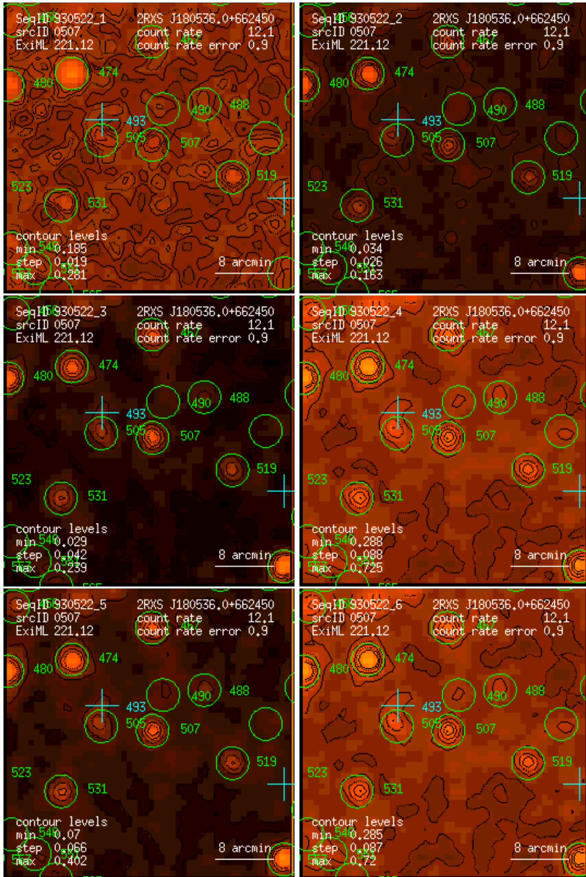
Figure 507: RASS 930522: detection 0507: band rate images, Gaussian filter: (1) PSPC channels 11 – 41, (2) 52 – 90, (3) 91 – 201, (4) 11 – 235, (5) 52 – 201, (6) 11 – 201. Broad band rates in counts/ks. Band rate contour levels in counts/ks/arcmin 2 .
