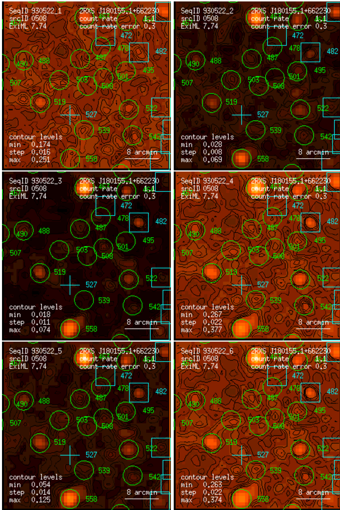
Figure 508: RASS 930522: detection 0508: band rate images, Gaussian filter: (1) PSPC channels 11 – 41, (2) 52 – 90, (3) 91 – 201, (4) 11 – 235, (5) 52 – 201, (6) 11 – 201. Broad band rates in counts/ks. Band rate contour levels in counts/ks/arcmin 2 .
