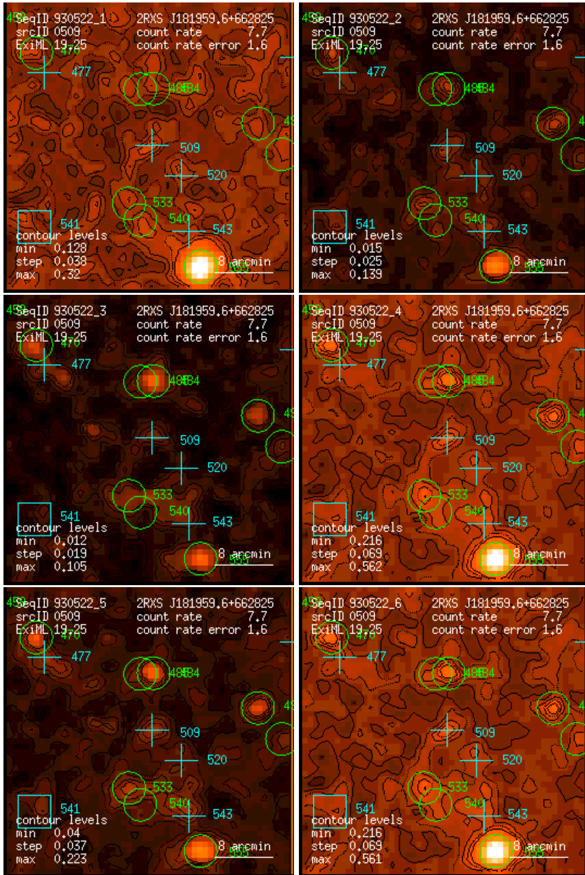
Figure 509: RASS 930522: detection 0509: band rate images, Gaussian filter: (1) PSPC channels 11 – 41, (2) 52 – 90, (3) 91 – 201, (4) 11 – 235, (5) 52 – 201, (6) 11 – 201. Broad band rates in counts/ks. Band rate contour levels in counts/ks/arcmin 2 .
