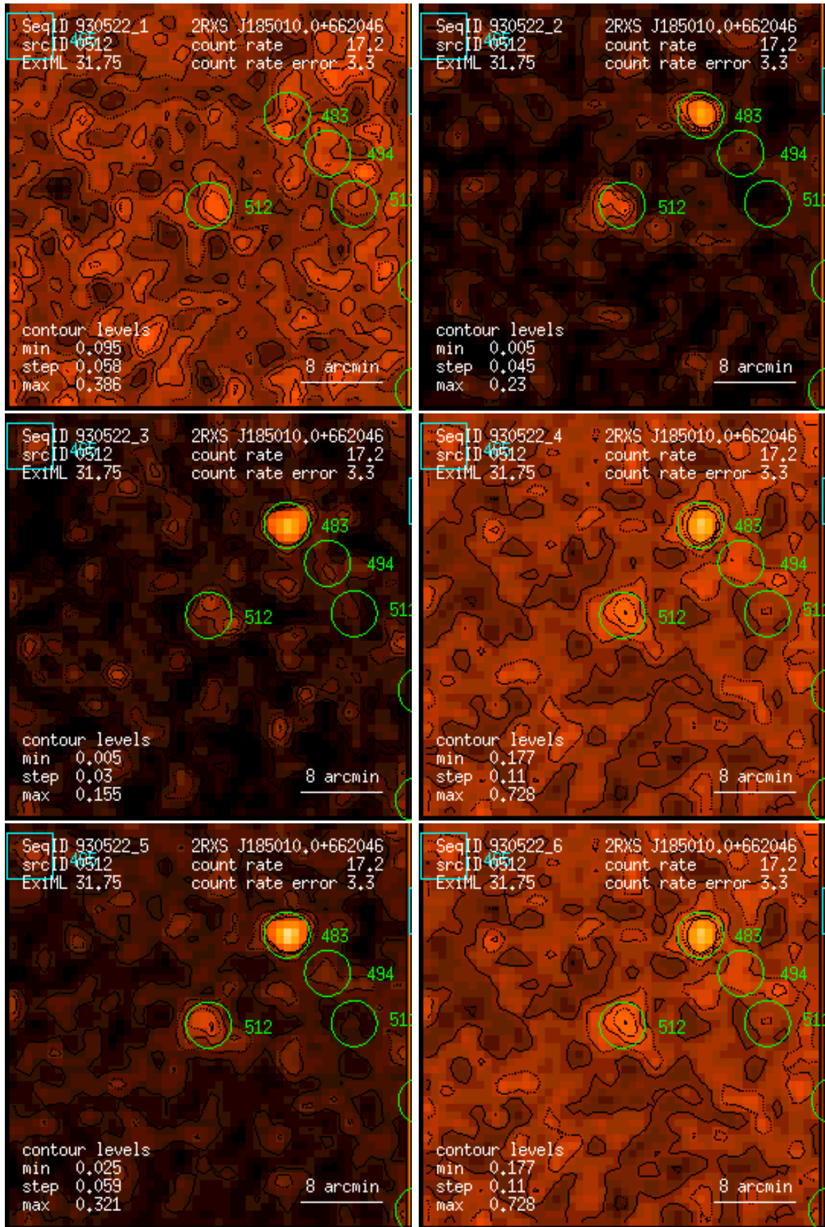
Figure 512: RASS 930522: detection 0512: band rate images, Gaussian filter: (1) PSPC channels 11 – 41, (2) 52 – 90, (3) 91 – 201, (4) 11 – 235, (5) 52 – 201, (6) 11 – 201. Broad band rates in counts/ks. Band rate contour levels in counts/ks/arcmin 2 .
