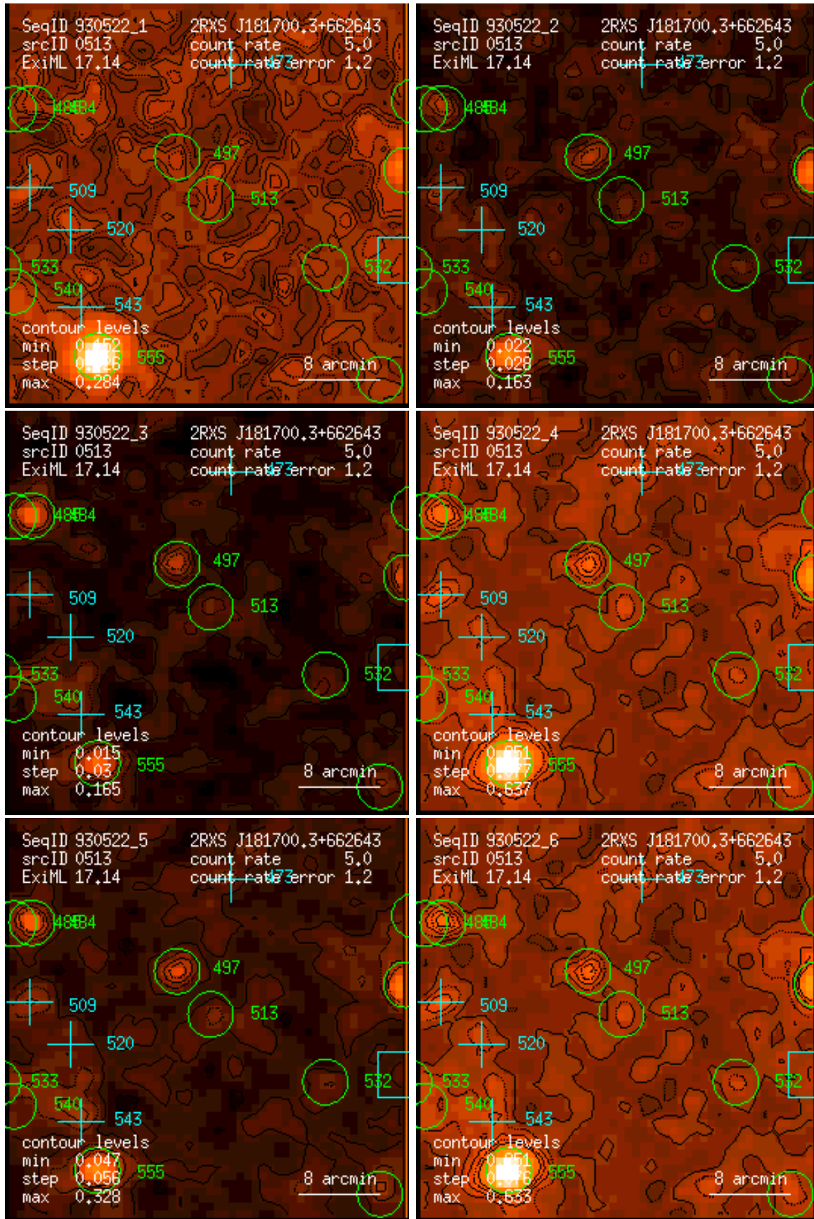
Figure 513: RASS 930522: detection 0513: band rate images, Gaussian filter: (1) PSPC channels 11 – 41, (2) 52 – 90, (3) 91 – 201, (4) 11 – 235, (5) 52 – 201, (6) 11 – 201. Broad band rates in counts/ks. Band rate contour levels in counts/ks/arcmin 2 .
