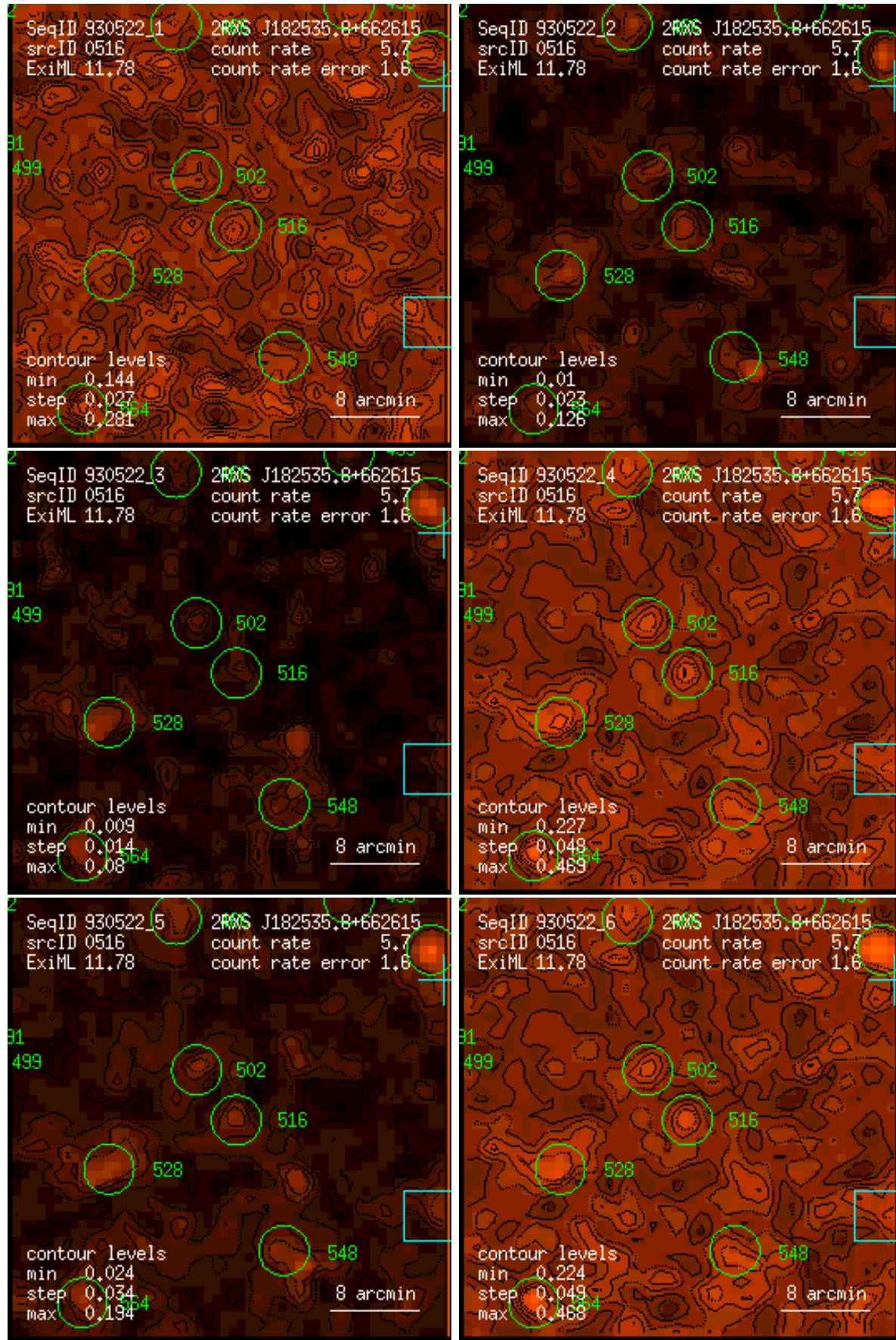
Figure 516: RASS 930522: detection 0516: band rate images, Gaussian filter: (1) PSPC channels 11 – 41, (2) 52 – 90, (3) 91 – 201, (4) 11 – 235, (5) 52 – 201, (6) 11 – 201. Broad band rates in counts/ks. Band rate contour levels in counts/ks/arcmin 2 .
