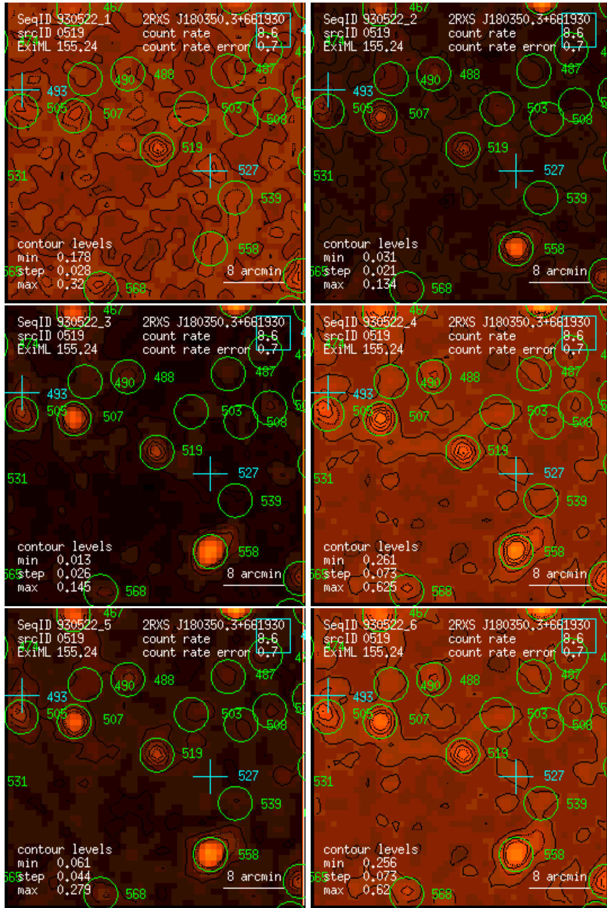
Figure 519: RASS 930522: detection 0519: band rate images, Gaussian filter: (1) PSPC channels 11 – 41, (2) 52 – 90, (3) 91 – 201, (4) 11 – 235, (5) 52 – 201, (6) 11 – 201. Broad band rates in counts/ks. Band rate contour levels in counts/ks/arcmin 2 .
