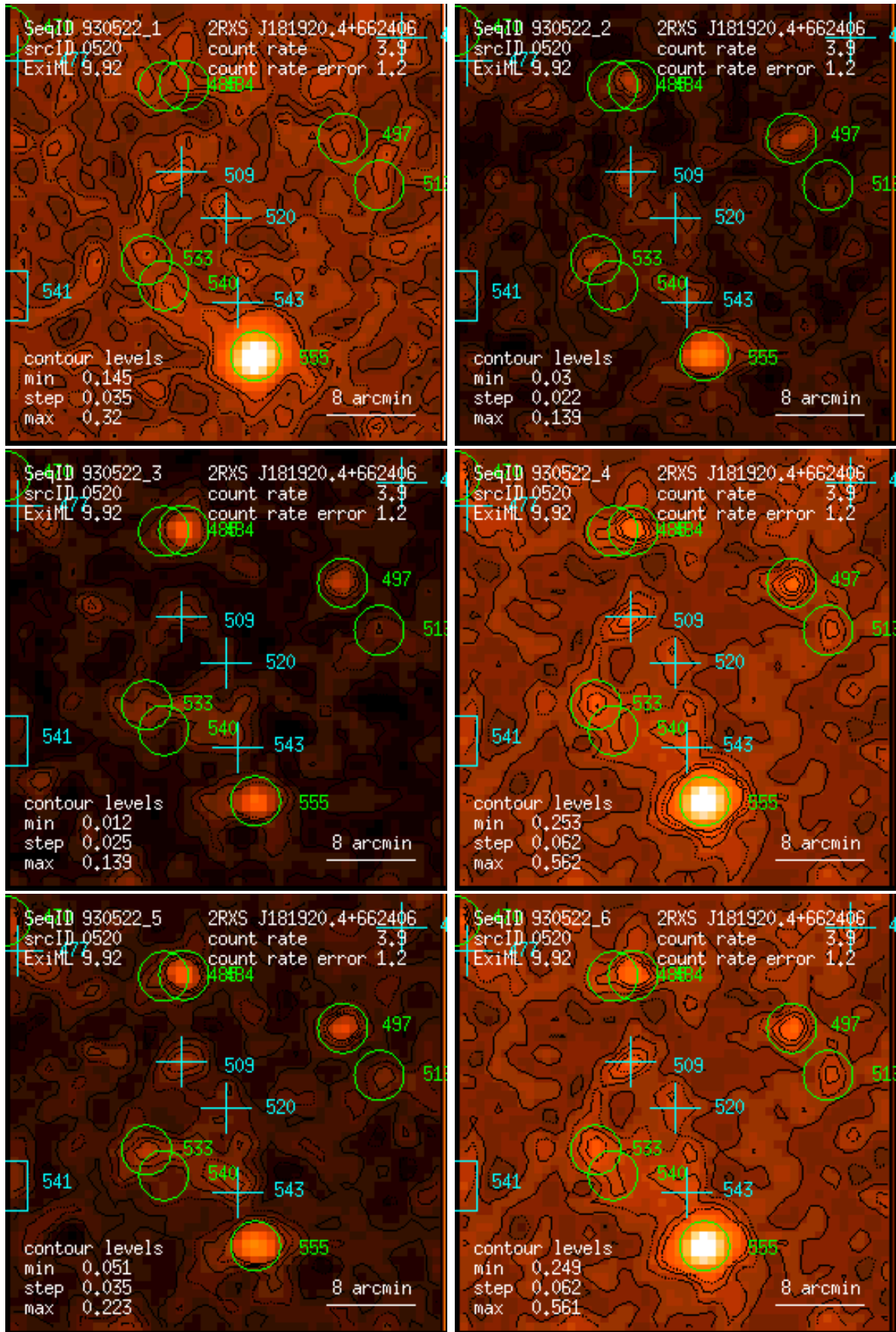
Figure 520: RASS 930522: detection 0520: band rate images, Gaussian filter: (1) PSPC channels 11 – 41, (2) 52 – 90, (3) 91 – 201, (4) 11 – 235, (5) 52 – 201, (6) 11 – 201. Broad band rates in counts/ks. Band rate contour levels in counts/ks/arcmin 2 .
