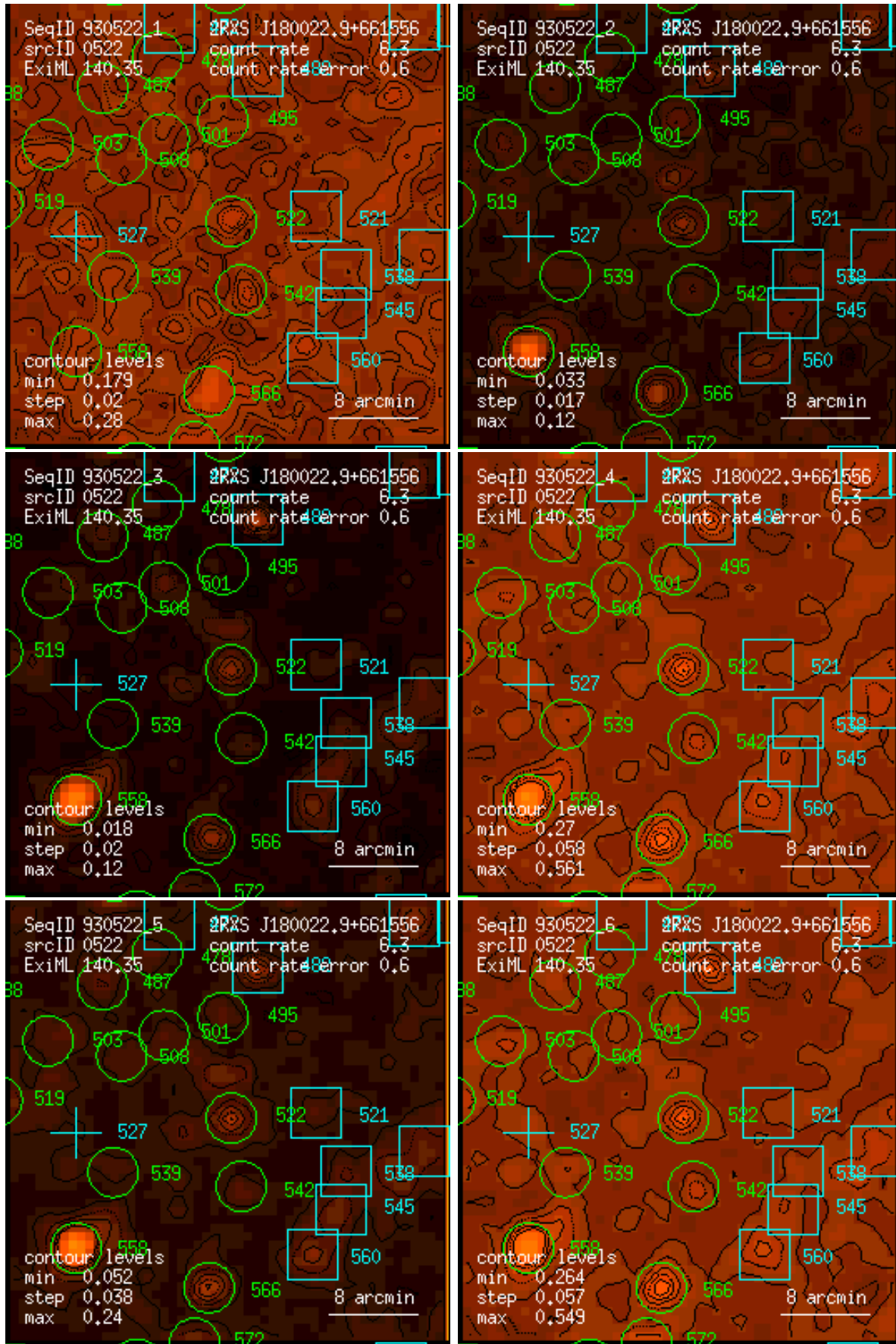
Figure 522: RASS 930522: detection 0522: band rate images, Gaussian filter: (1) PSPC channels 11 – 41, (2) 52 – 90, (3) 91 – 201, (4) 11 – 235, (5) 52 – 201, (6) 11 – 201. Broad band rates in counts/ks. Band rate contour levels in counts/ks/arcmin 2 .
