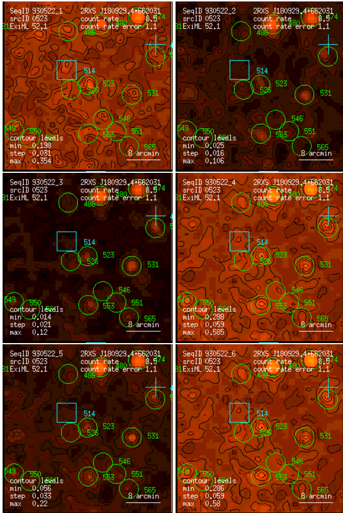
Figure 523: RASS 930522: detection 0523: band rate images, Gaussian filter: (1) PSPC channels 11 – 41, (2) 52 – 90, (3) 91 – 201, (4) 11 – 235, (5) 52 – 201, (6) 11 – 201. Broad band rates in counts/ks. Band rate contour levels in counts/ks/arcmin 2 .
