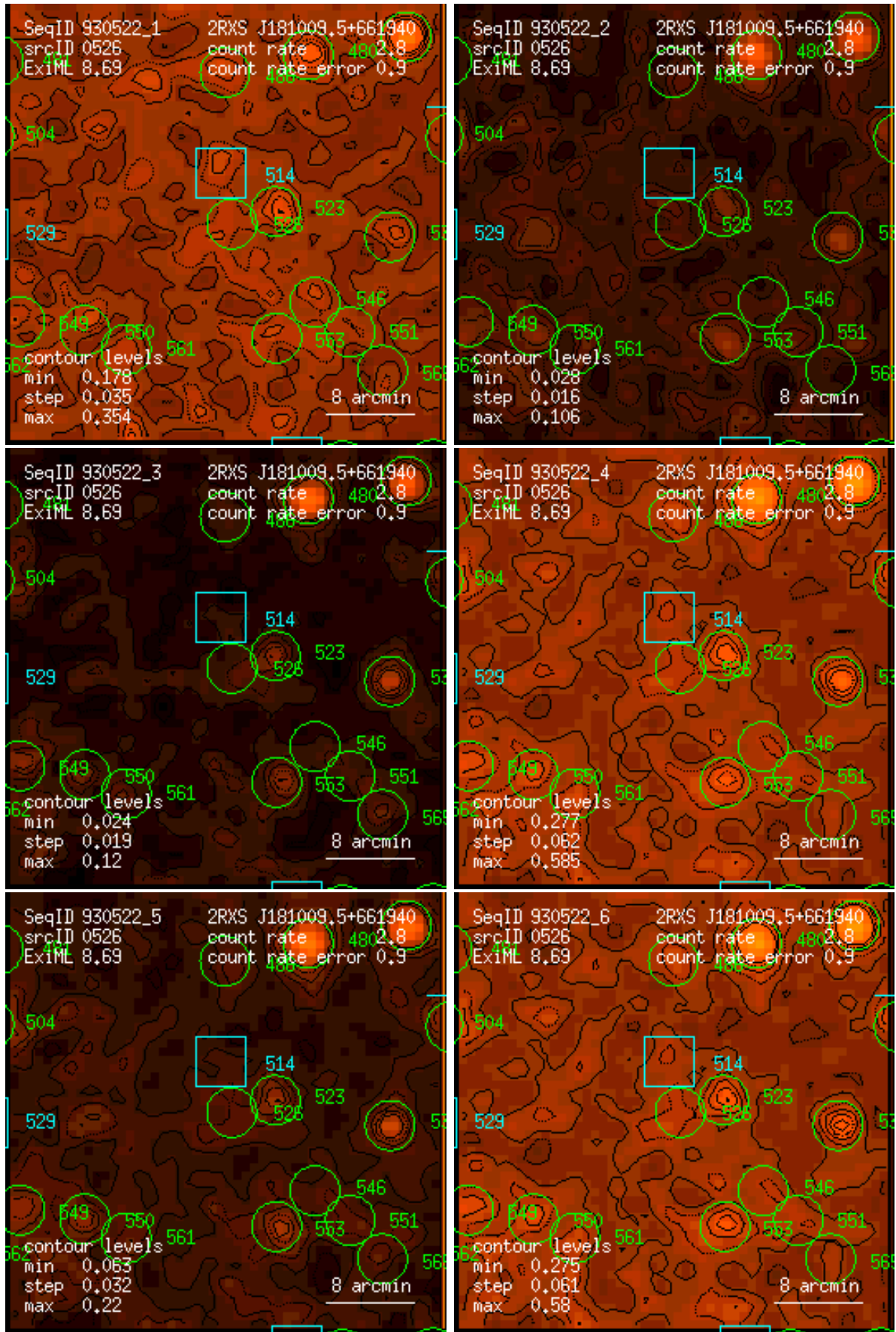
Figure 526: RASS 930522: detection 0526: band rate images, Gaussian filter: (1) PSPC channels 11 – 41, (2) 52 – 90, (3) 91 – 201, (4) 11 – 235, (5) 52 – 201, (6) 11 – 201. Broad band rates in counts/ks. Band rate contour levels in counts/ks/arcmin 2 .
