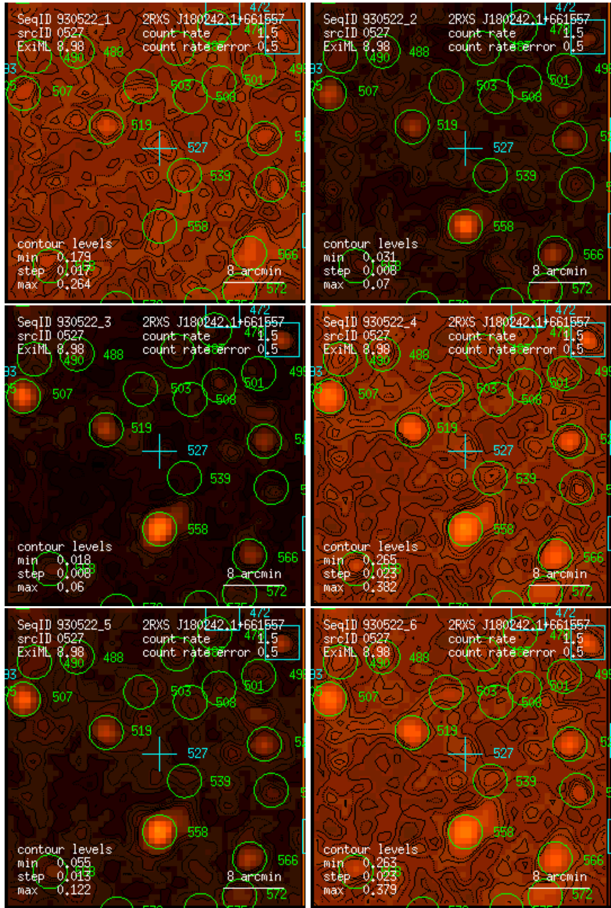
Figure 527: RASS 930522: detection 0527: band rate images, Gaussian filter: (1) PSPC channels 11 – 41, (2) 52 – 90, (3) 91 – 201, (4) 11 – 235, (5) 52 – 201, (6) 11 – 201. Broad band rates in counts/ks. Band rate contour levels in counts/ks/arcmin 2 .
