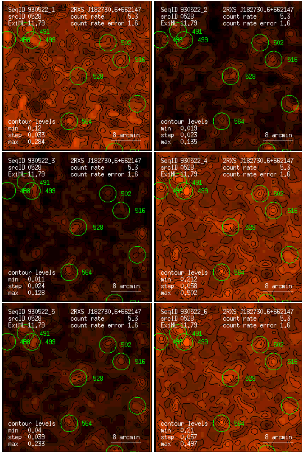
Figure 528: RASS 930522: detection 0528: band rate images, Gaussian filter: (1) PSPC channels 11 – 41, (2) 52 – 90, (3) 91 – 201, (4) 11 – 235, (5) 52 – 201, (6) 11 – 201. Broad band rates in counts/ks. Band rate contour levels in counts/ks/arcmin 2 .
