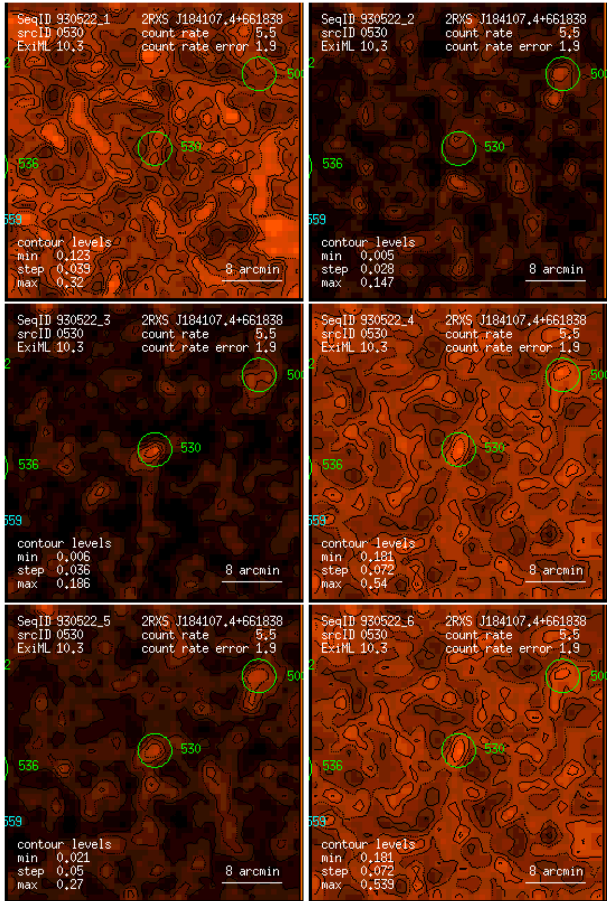
Figure 530: RASS 930522: detection 0530: band rate images, Gaussian filter: (1) PSPC channels 11 – 41, (2) 52 – 90, (3) 91 – 201, (4) 11 – 235, (5) 52 – 201, (6) 11 – 201. Broad band rates in counts/ks. Band rate contour levels in counts/ks/arcmin 2 .
