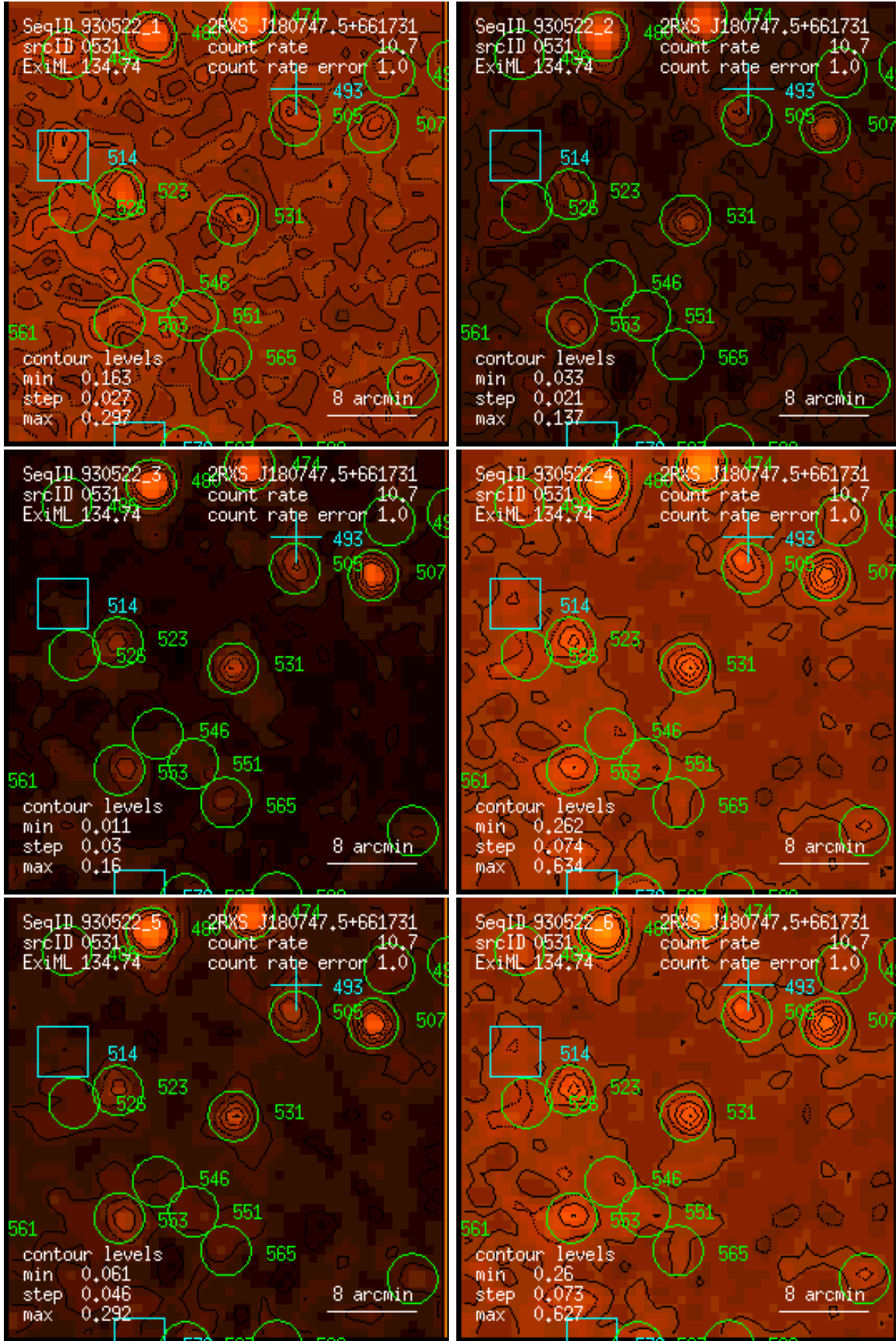
Figure 531: RASS 930522: detection 0531: band rate images, Gaussian filter: (1) PSPC channels 11 – 41, (2) 52 – 90, (3) 91 – 201, (4) 11 – 235, (5) 52 – 201, (6) 11 – 201. Broad band rates in counts/ks. Band rate contour levels in counts/ks/arcmin 2 .
