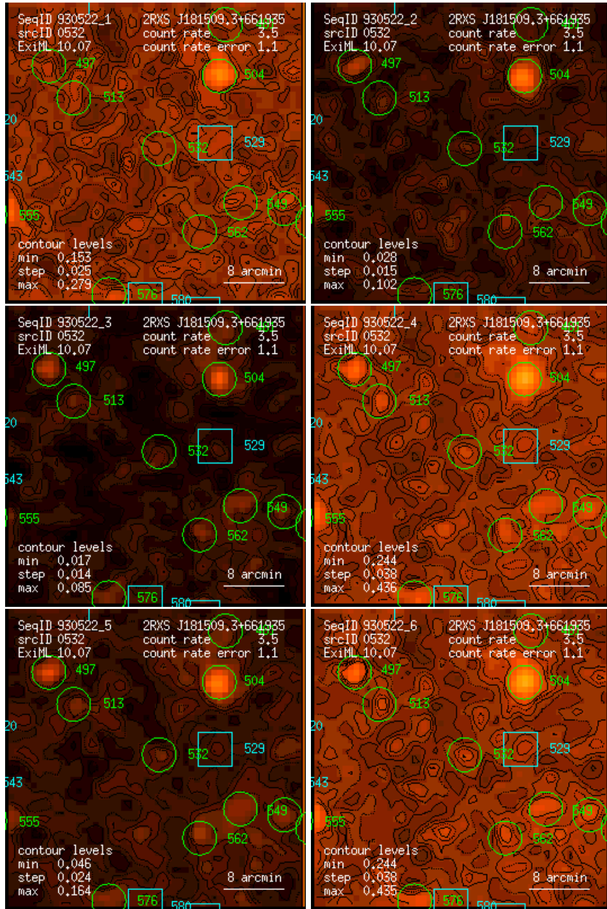
Figure 532: RASS 930522: detection 0532: band rate images, Gaussian filter: (1) PSPC channels 11 – 41, (2) 52 – 90, (3) 91 – 201, (4) 11 – 235, (5) 52 – 201, (6) 11 – 201. Broad band rates in counts/ks. Band rate contour levels in counts/ks/arcmin 2 .
