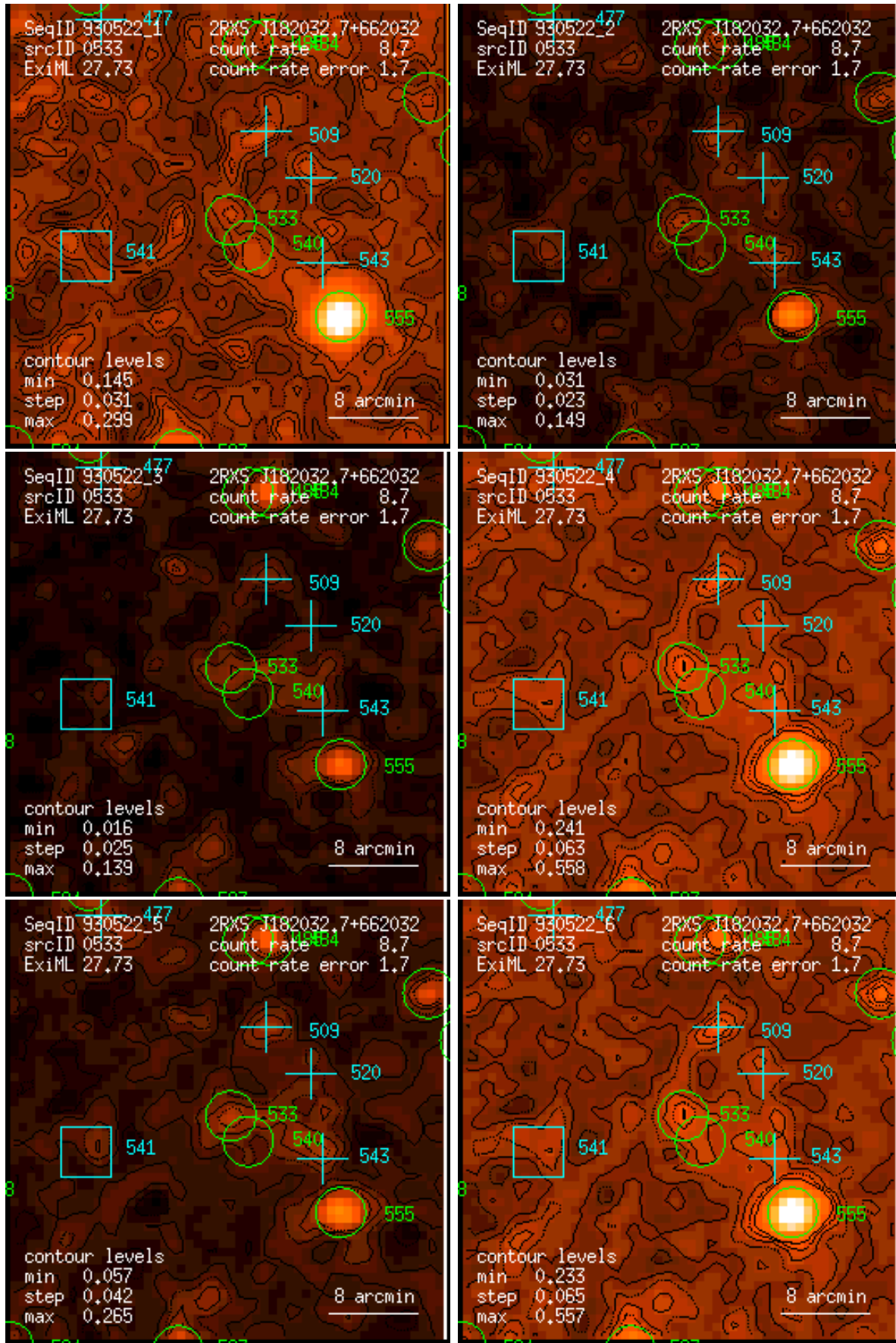
Figure 533: RASS 930522: detection 0533: band rate images, Gaussian filter: (1) PSPC channels 11 – 41, (2) 52 – 90, (3) 91 – 201, (4) 11 – 235, (5) 52 – 201, (6) 11 – 201. Broad band rates in counts/ks. Band rate contour levels in counts/ks/arcmin 2 .
