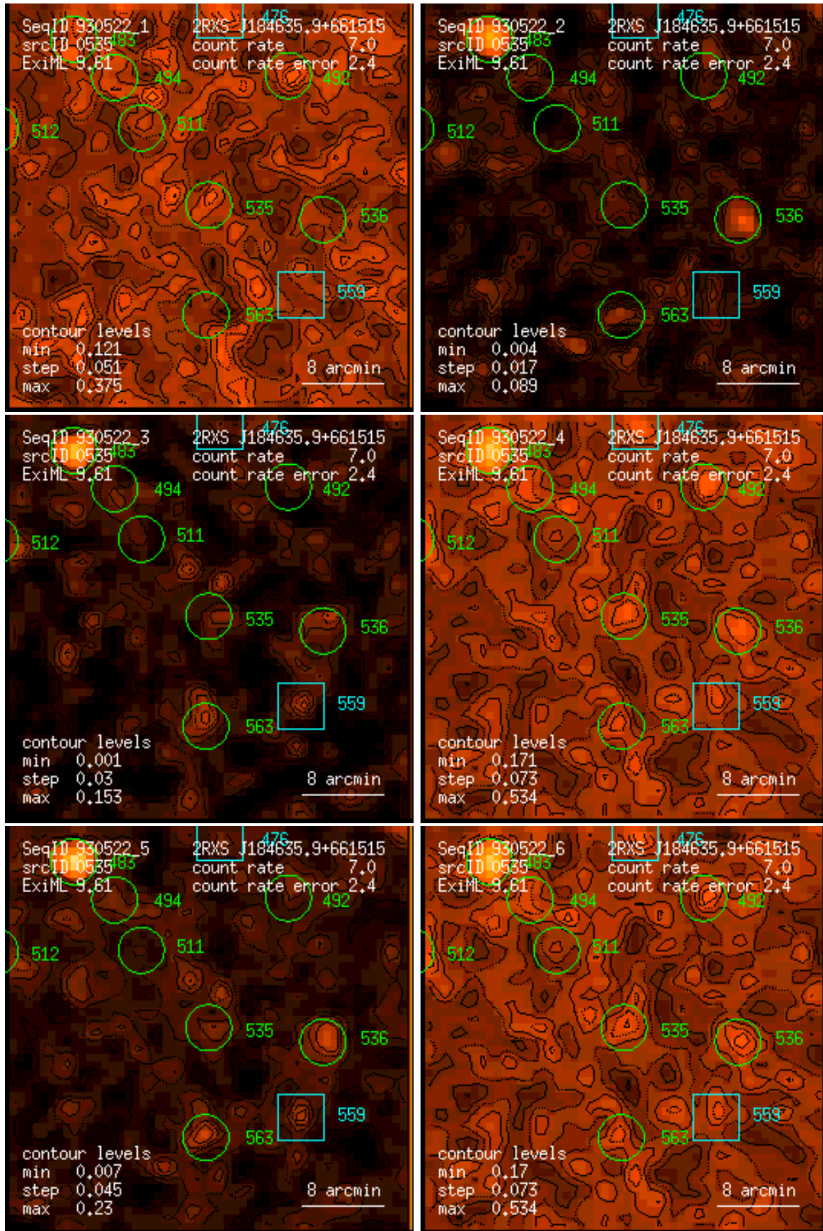
Figure 535: RASS 930522: detection 0535: band rate images, Gaussian filter: (1) PSPC channels 11 – 41, (2) 52 – 90, (3) 91 – 201, (4) 11 – 235, (5) 52 – 201, (6) 11 – 201. Broad band rates in counts/ks. Band rate contour levels in counts/ks/arcmin 2 .
