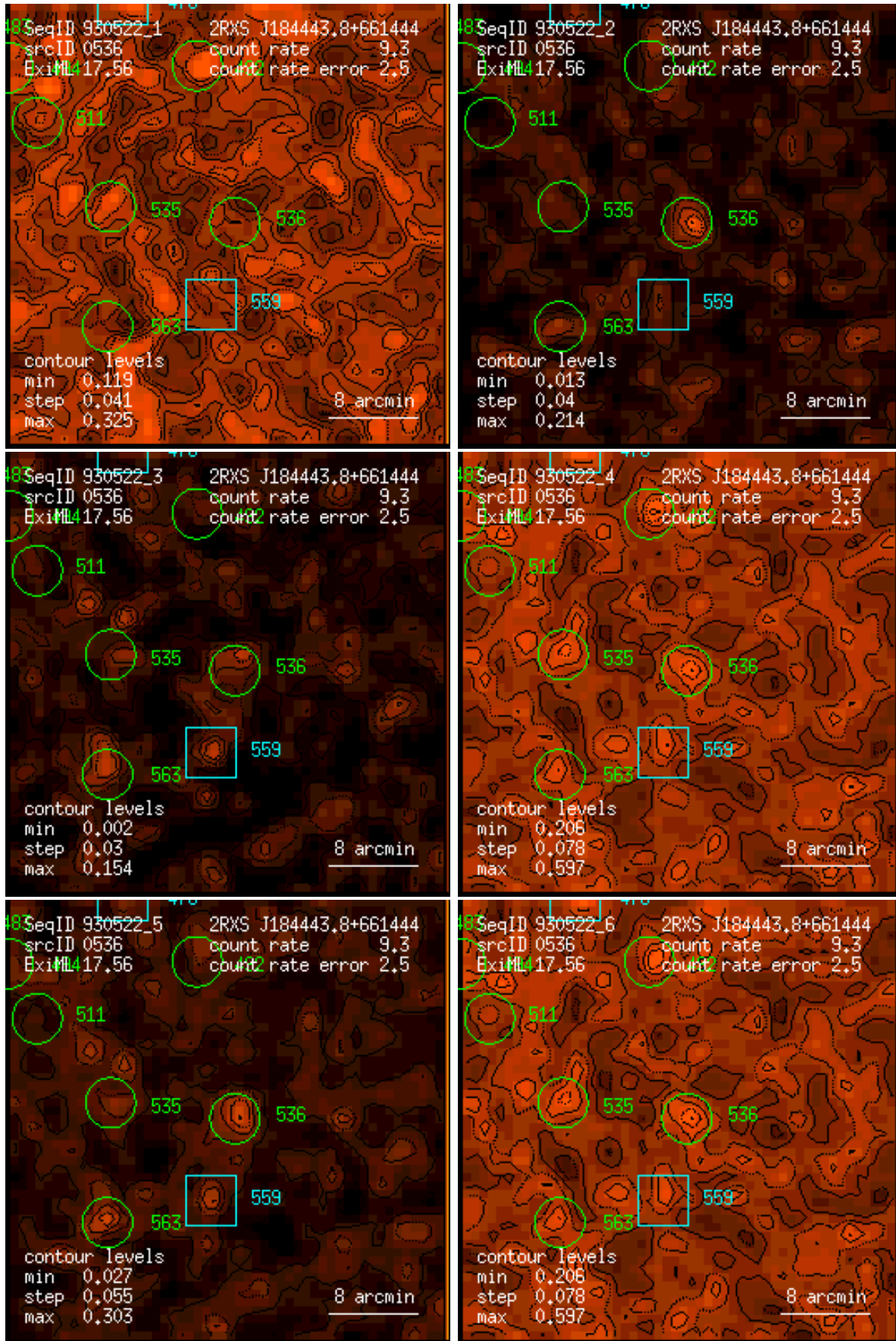
Figure 536: RASS 930522: detection 0536: band rate images, Gaussian filter: (1) PSPC channels 11 – 41, (2) 52 – 90, (3) 91 – 201, (4) 11 – 235, (5) 52 – 201, (6) 11 – 201. Broad band rates in counts/ks. Band rate contour levels in counts/ks/arcmin 2 .
