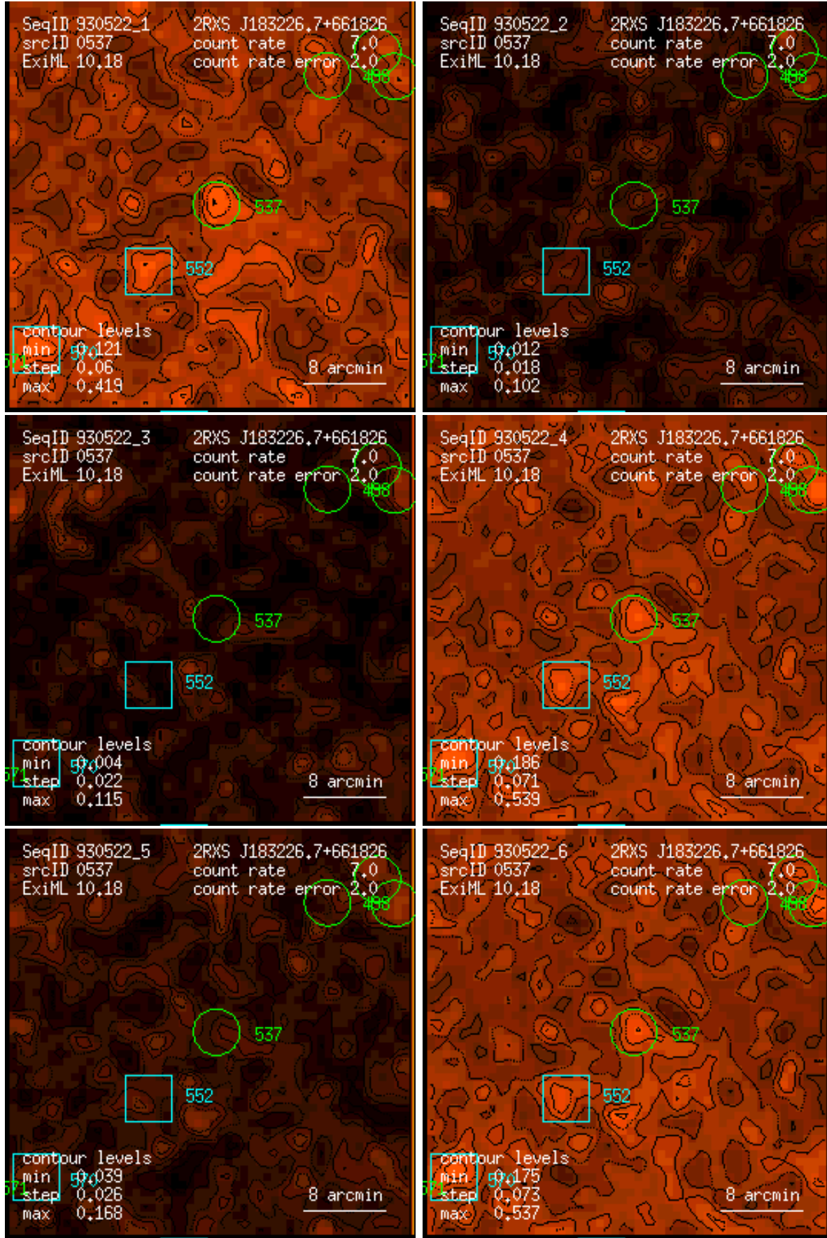
Figure 537: RASS 930522: detection 0537: band rate images, Gaussian filter: (1) PSPC channels 11 – 41, (2) 52 – 90, (3) 91 – 201, (4) 11 – 235, (5) 52 – 201, (6) 11 – 201. Broad band rates in counts/ks. Band rate contour levels in counts/ks/arcmin 2 .
