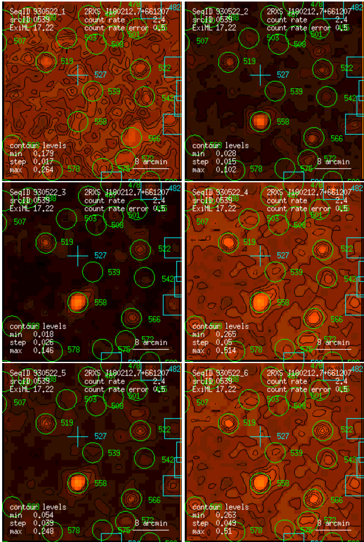
Figure 539: RASS 930522: detection 0539: band rate images, Gaussian filter: (1) PSPC channels 11 – 41, (2) 52 – 90, (3) 91 – 201, (4) 11 – 235, (5) 52 – 201, (6) 11 – 201. Broad band rates in counts/ks. Band rate contour levels in counts/ks/arcmin 2 .
