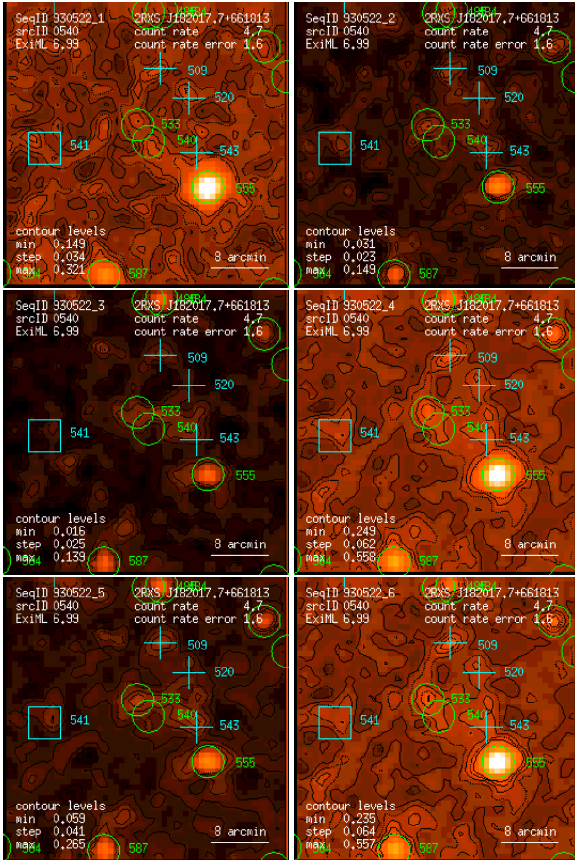
Figure 540: RASS 930522: detection 0540: band rate images, Gaussian filter: (1) PSPC channels 11 – 41, (2) 52 – 90, (3) 91 – 201, (4) 11 – 235, (5) 52 – 201, (6) 11 – 201. Broad band rates in counts/ks. Band rate contour levels in counts/ks/arcmin 2 .
